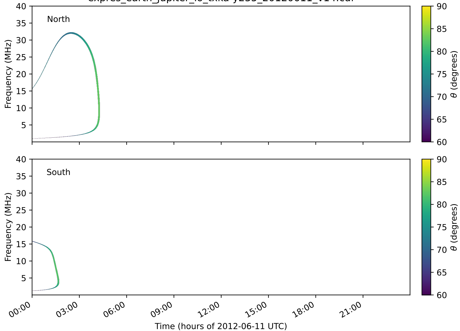
expres_earth_jupiter_io_txka-y235_20120611_v14.cdf
