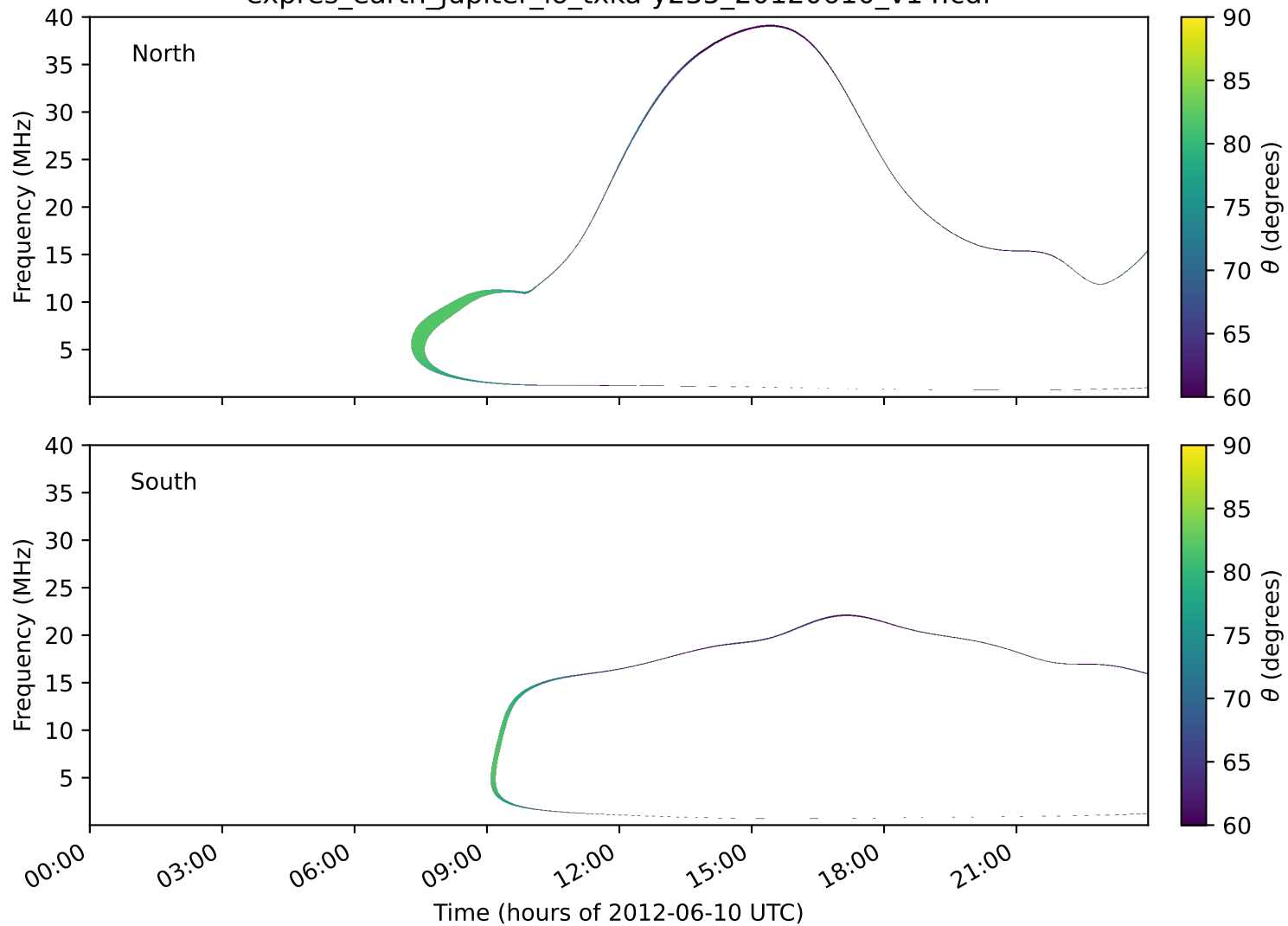
expres_earth_jupiter_io_txka-y235_20120610_v14.cdf
