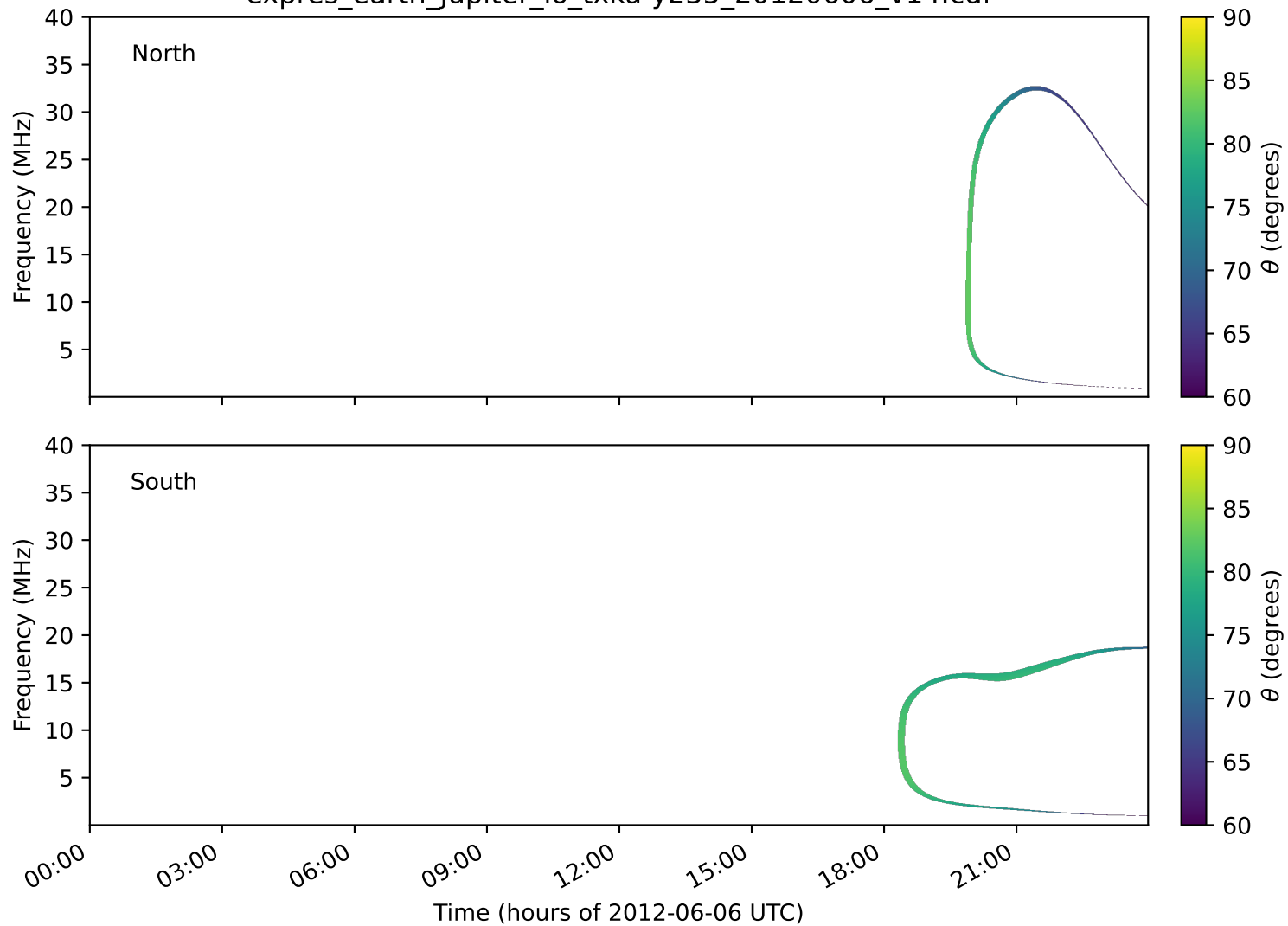
expres_earth_jupiter_io_txka-y235_20120606_v14.cdf
