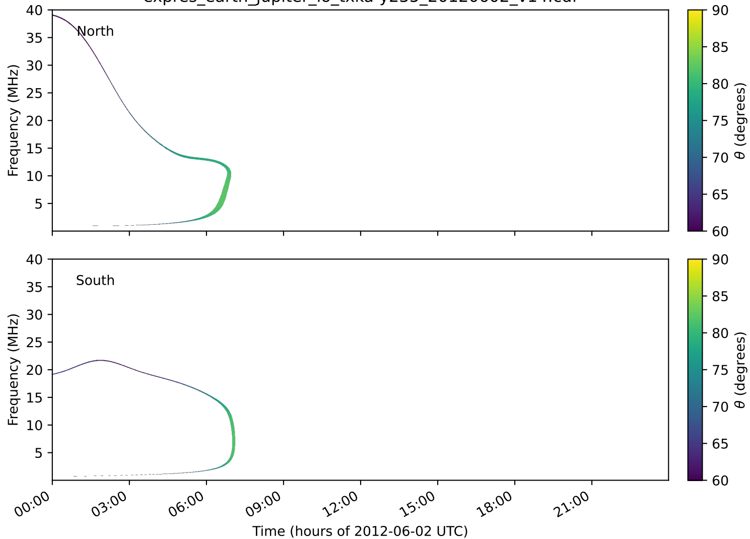
expres_earth_jupiter_io_txka-y235_20120602_v14.cdf
