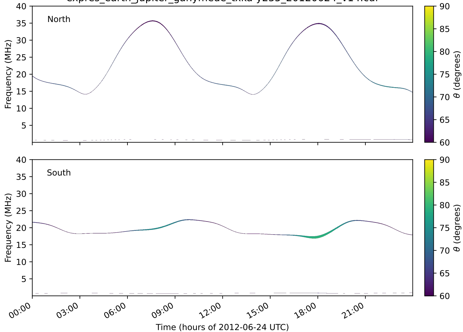
expres_earth_jupiter_ganymede_txka-y235_20120624_v14.cdf
