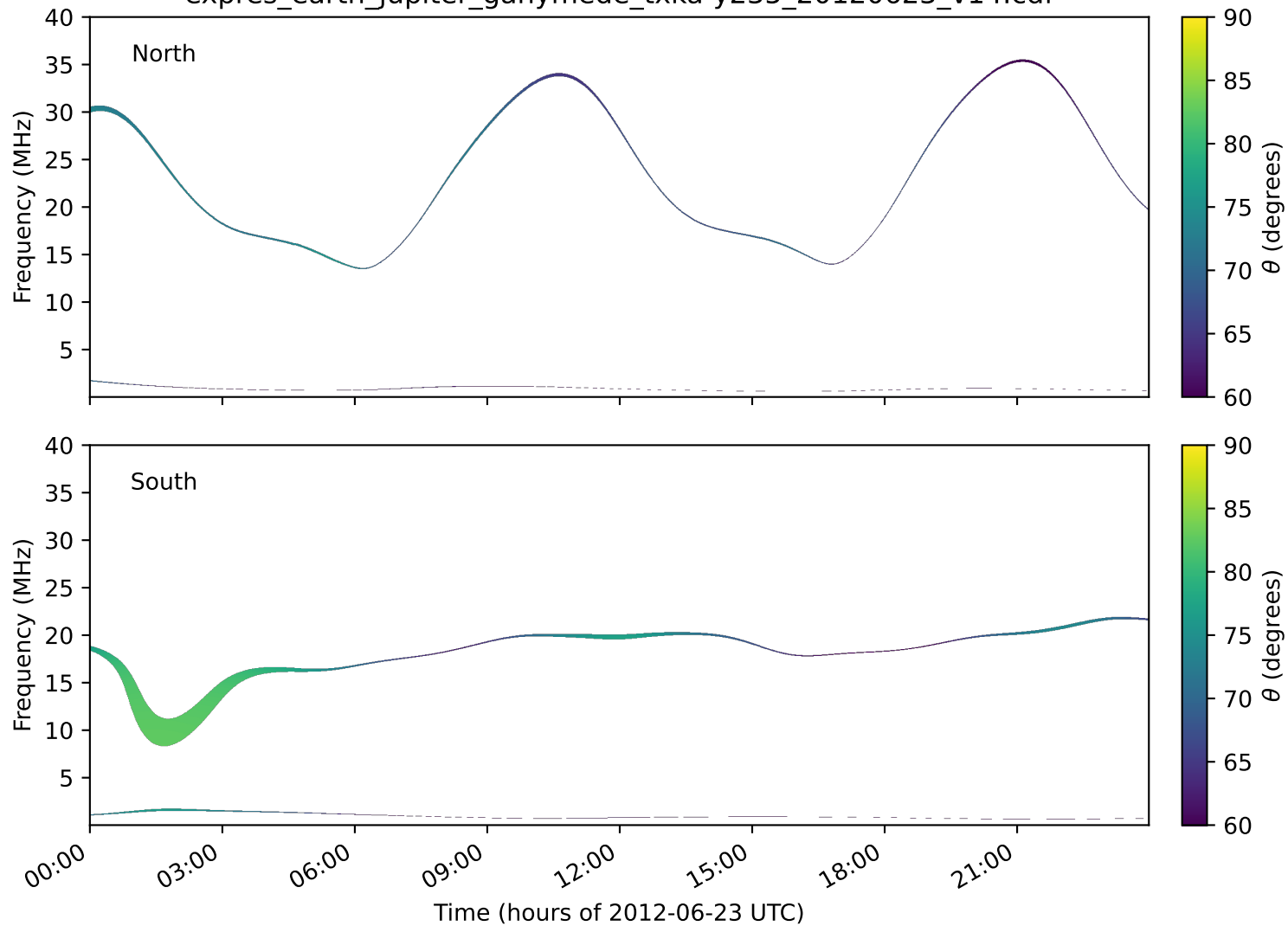
expres_earth_jupiter_ganymede_txka-y235_20120623_v14.cdf
