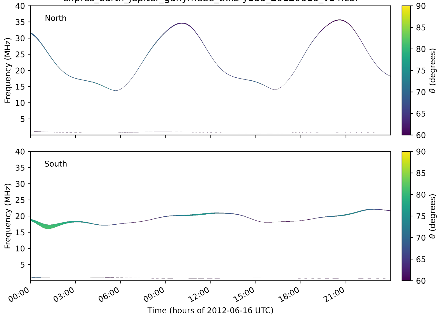
expres_earth_jupiter_ganymede_txka-y235_20120616_v14.cdf
