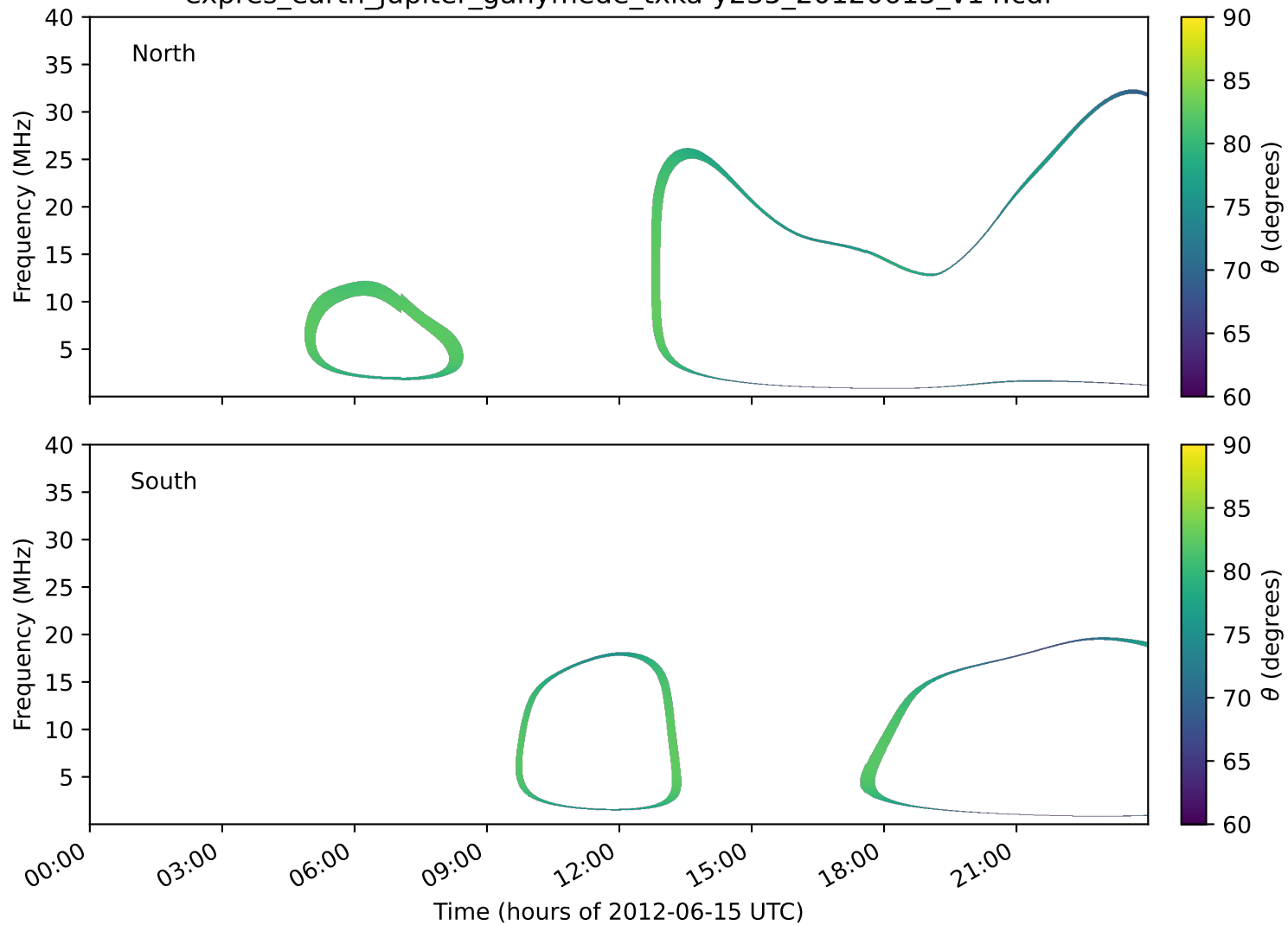
expres_earth_jupiter_ganymede_txka-y235_20120615_v14.cdf
