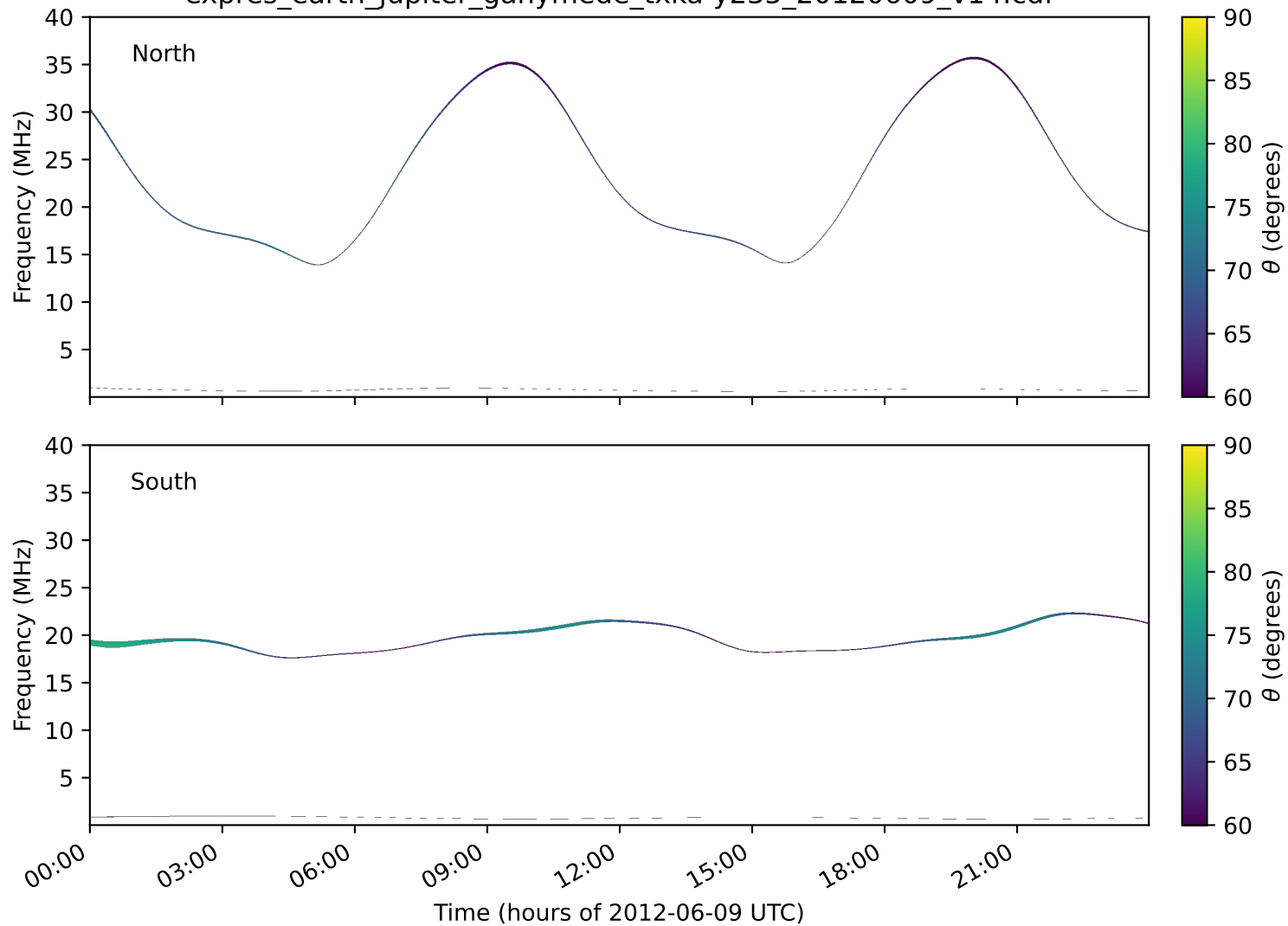
expres_earth_jupiter_ganymede_txka-y235_20120609_v14.cdf
