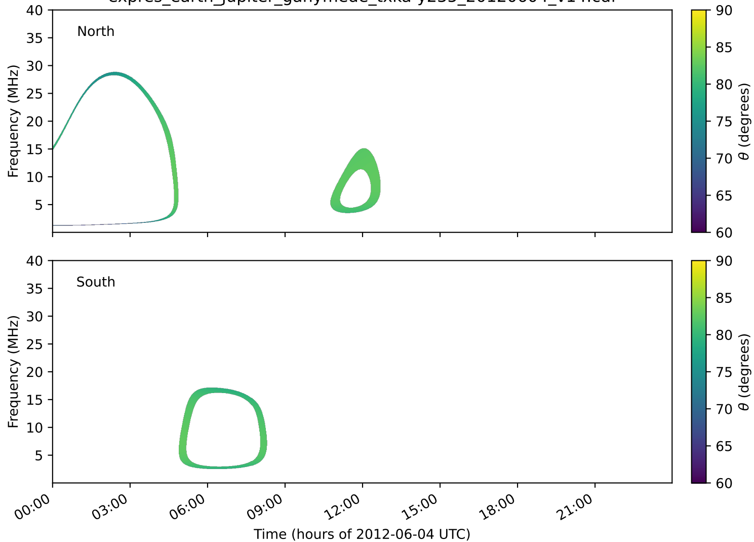
expres_earth_jupiter_ganymede_txka-y235_20120604_v14.cdf
