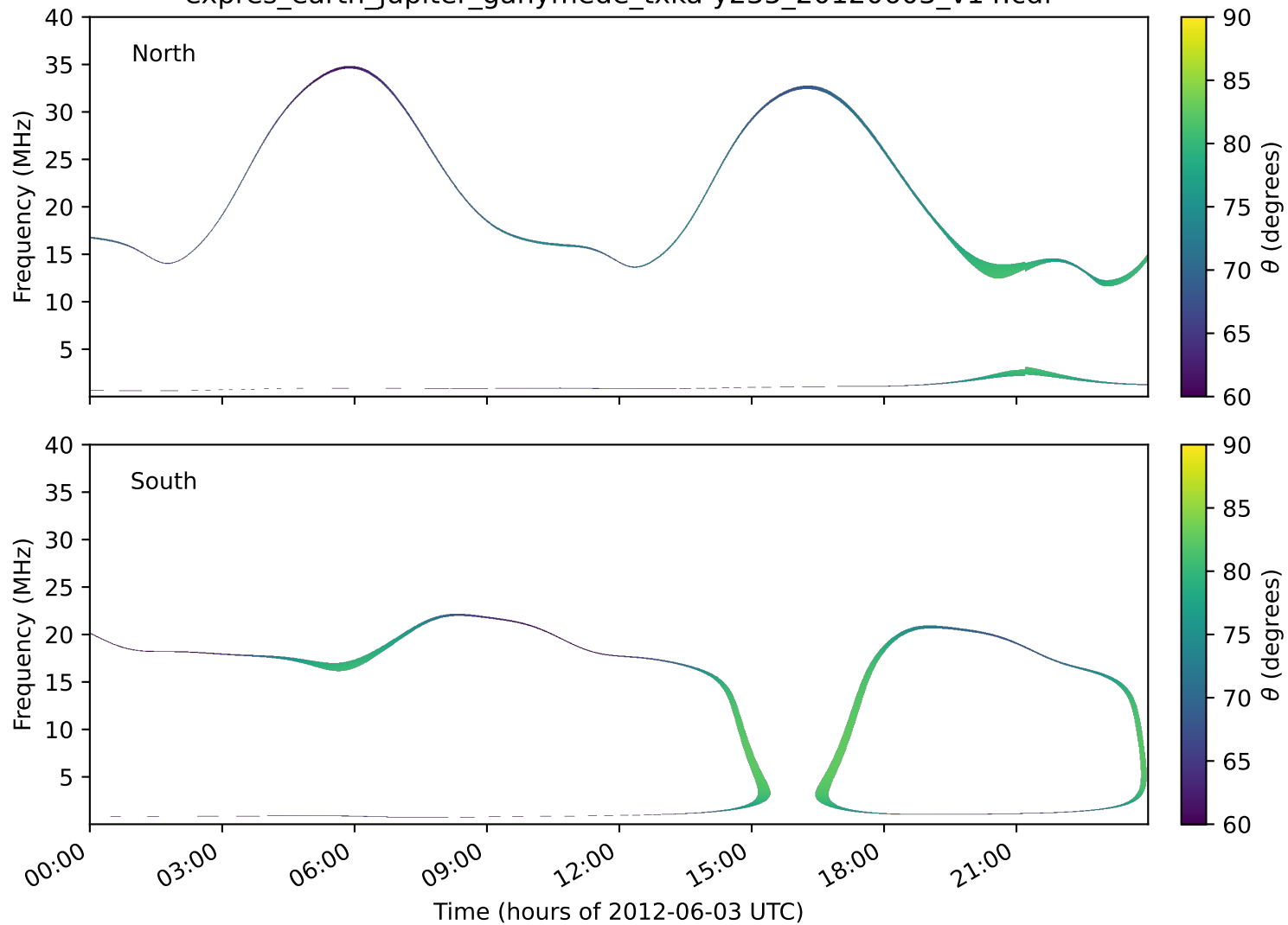
expres_earth_jupiter_ganymede_txka-y235_20120603_v14.cdf
