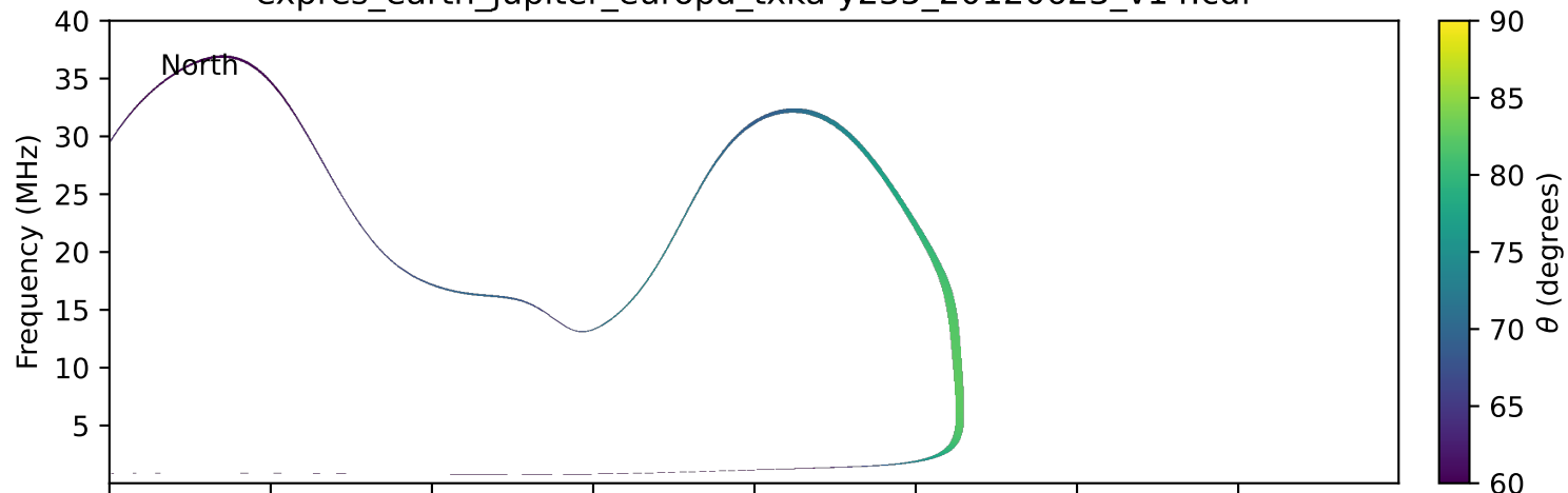
expres_earth_jupiter_europa_txka-y235_20120623_v14.cdf
