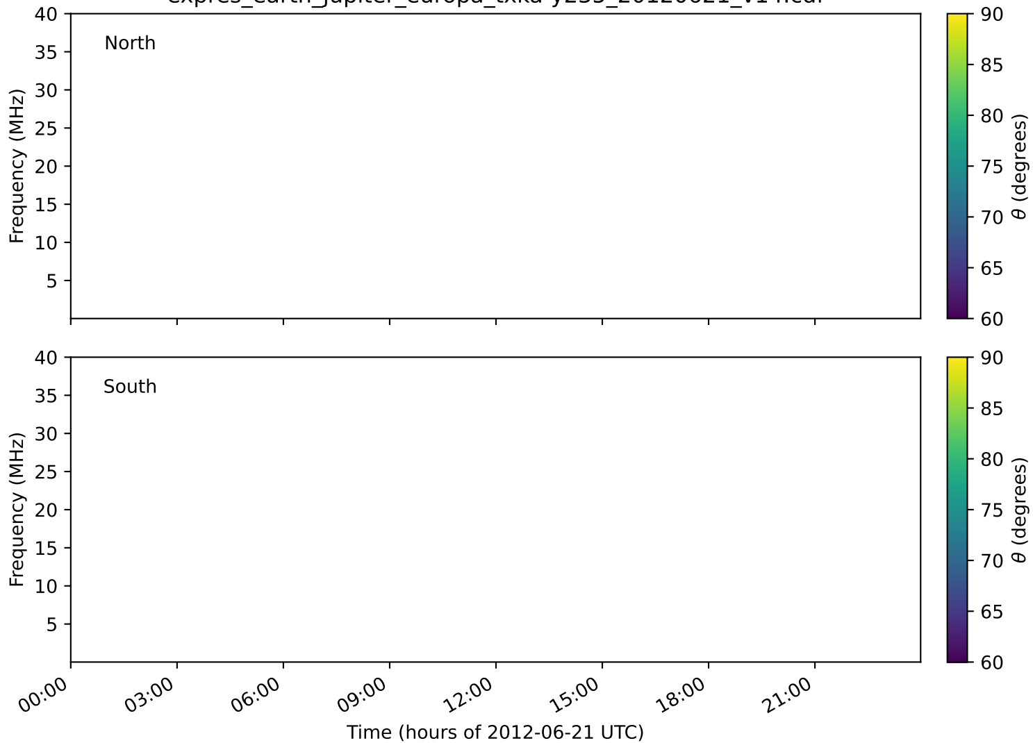
expres_earth_jupiter_europa_txka-y235_20120621_v14.cdf
