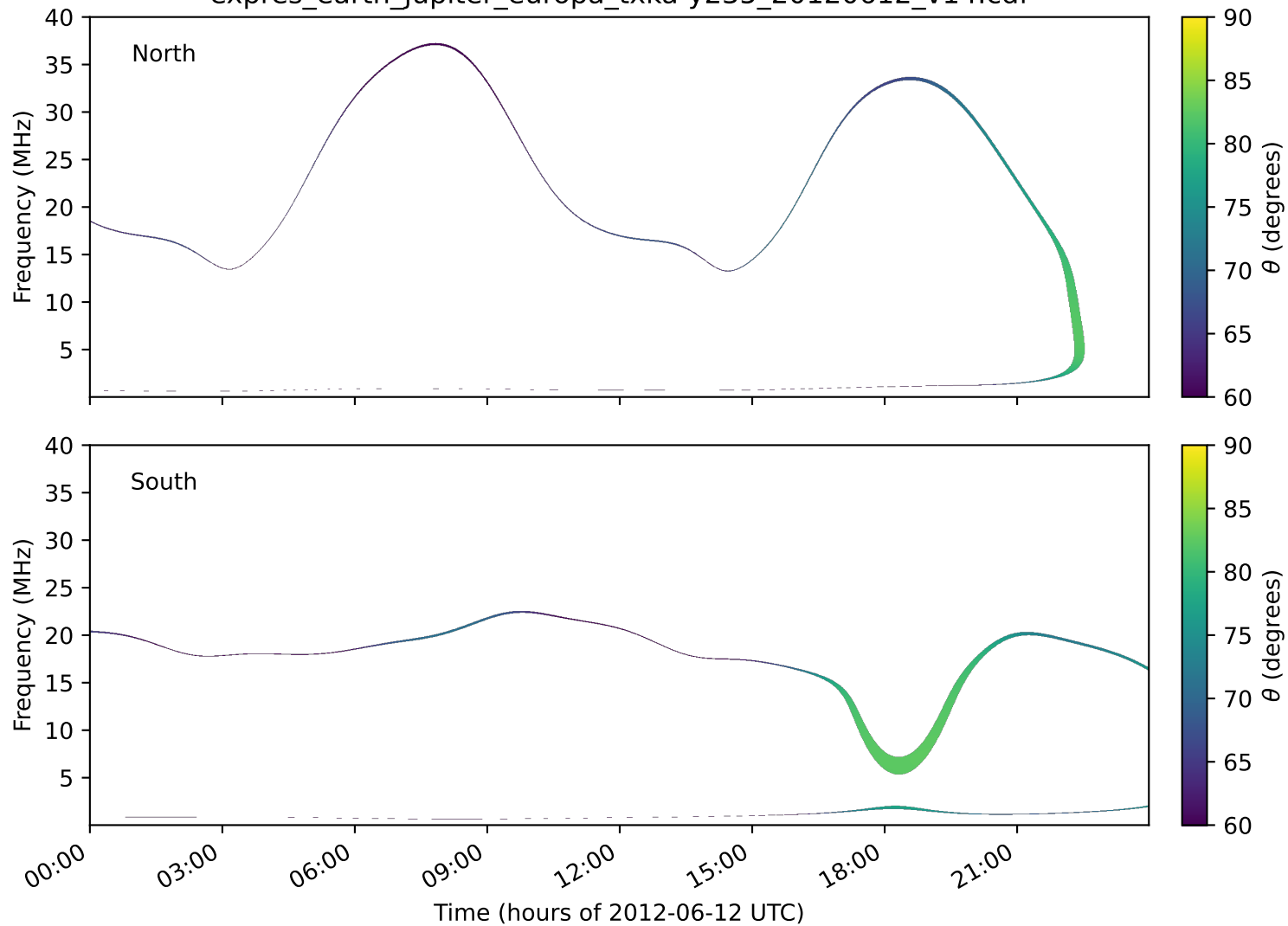
expres_earth_jupiter_europa_txka-y235_20120612_v14.cdf
