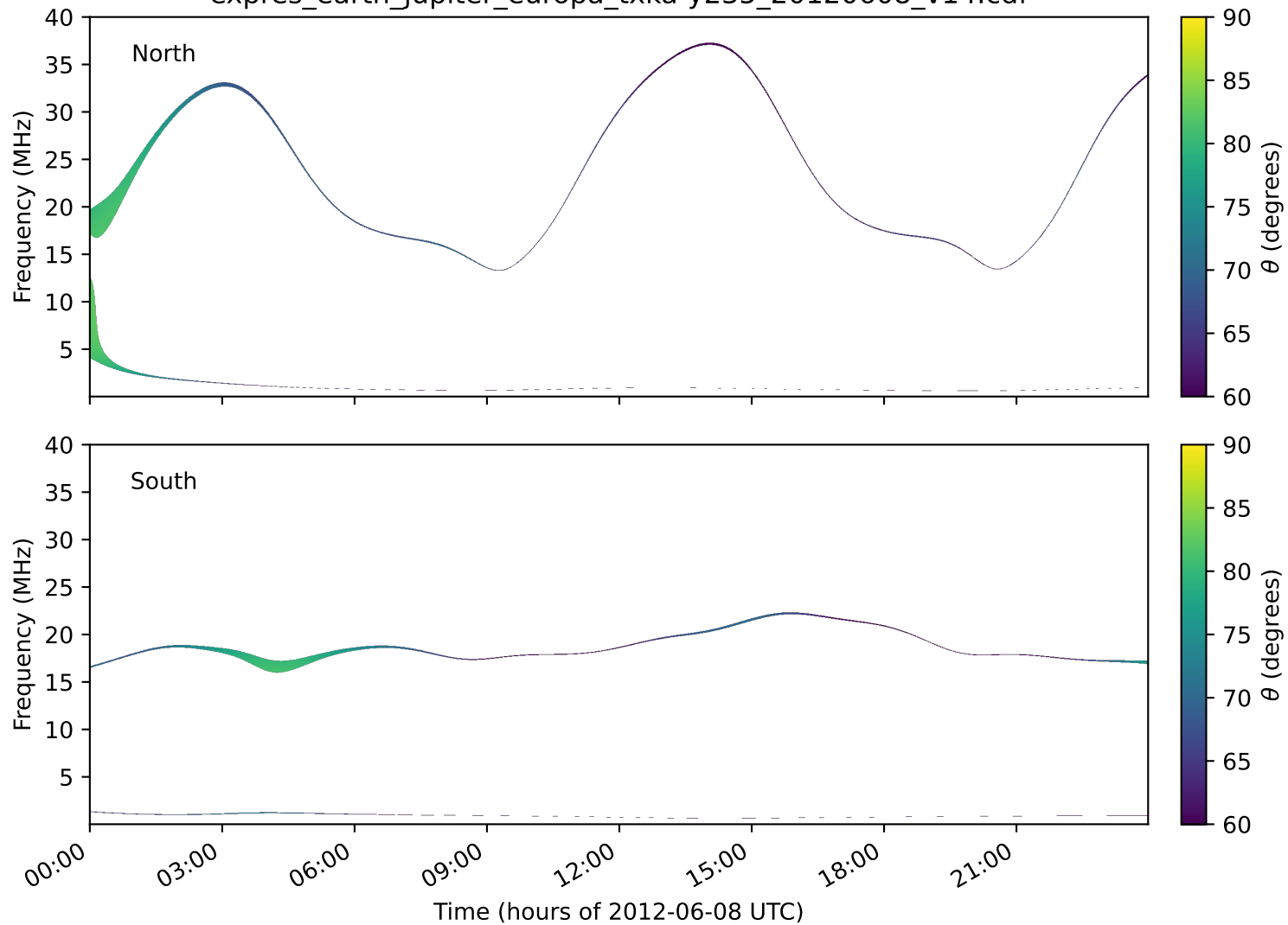
expres_earth_jupiter_europa_txka-y235_20120608_v14.cdf
