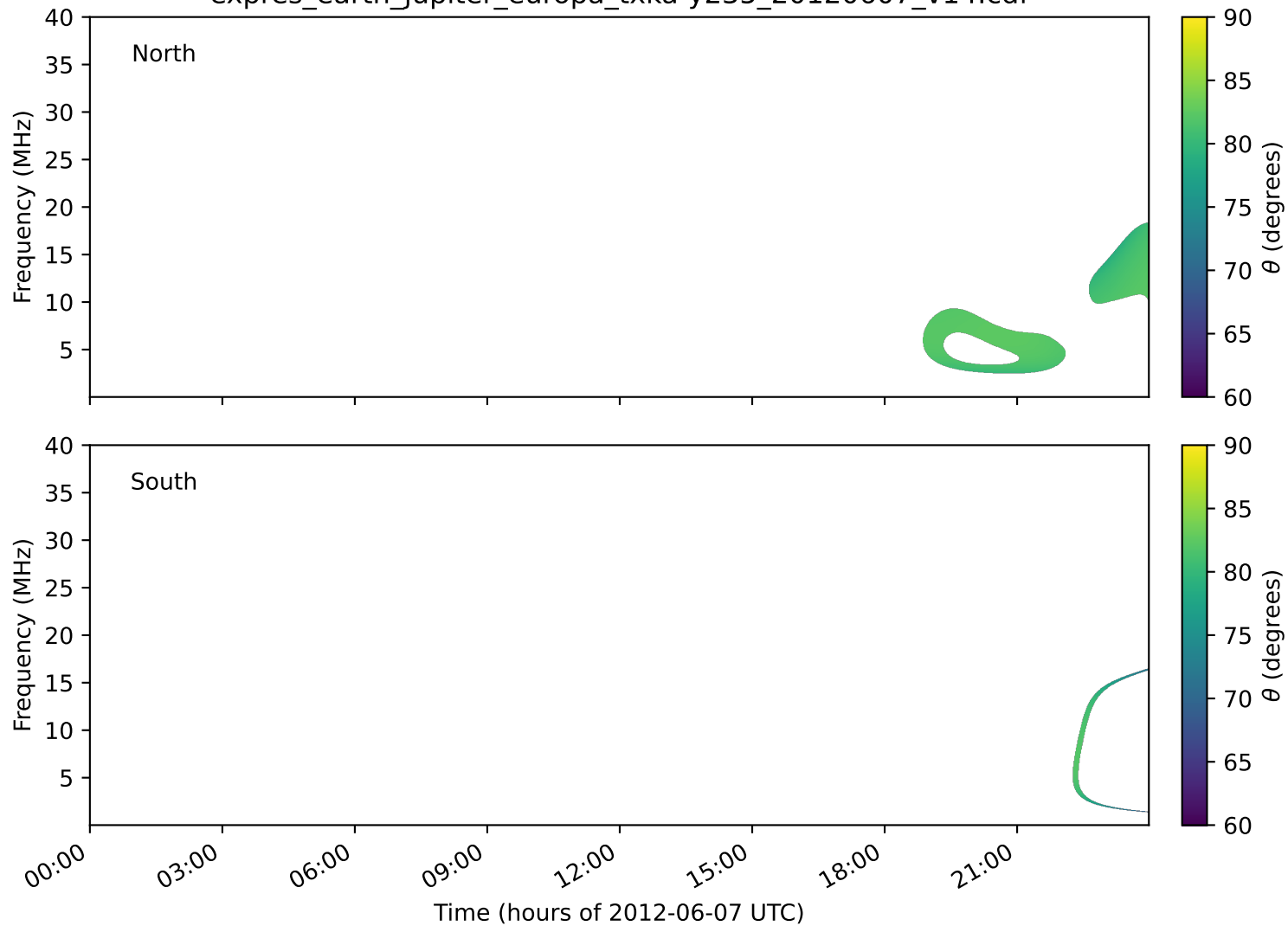
expres_earth_jupiter_europa_txka-y235_20120607_v14.cdf
