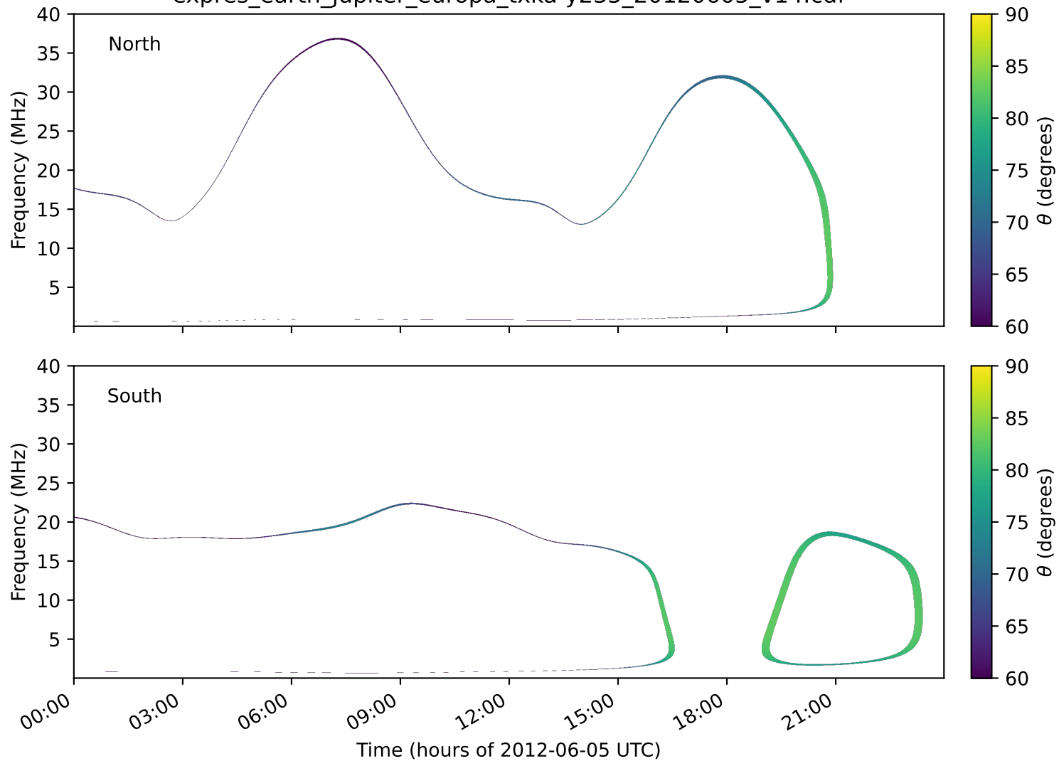
expres_earth_jupiter_europa_txka-y235_20120605_v14.cdf
