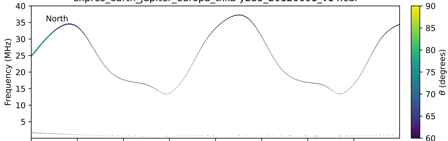
expres_earth_jupiter_europa_txka-y235_20120601_v14.cdf
