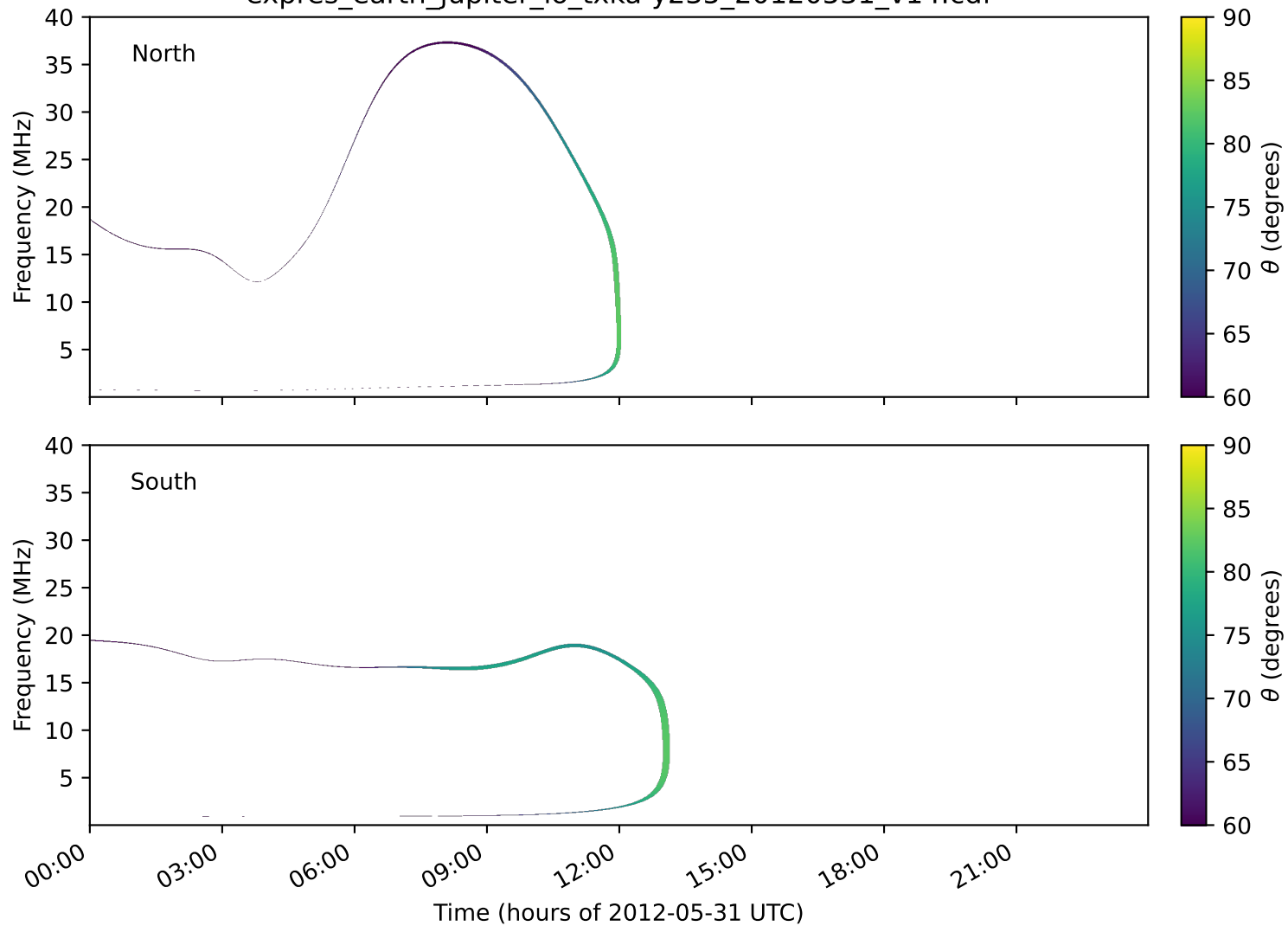
expres_earth_jupiter_io_txka-y235_20120531_v14.cdf
