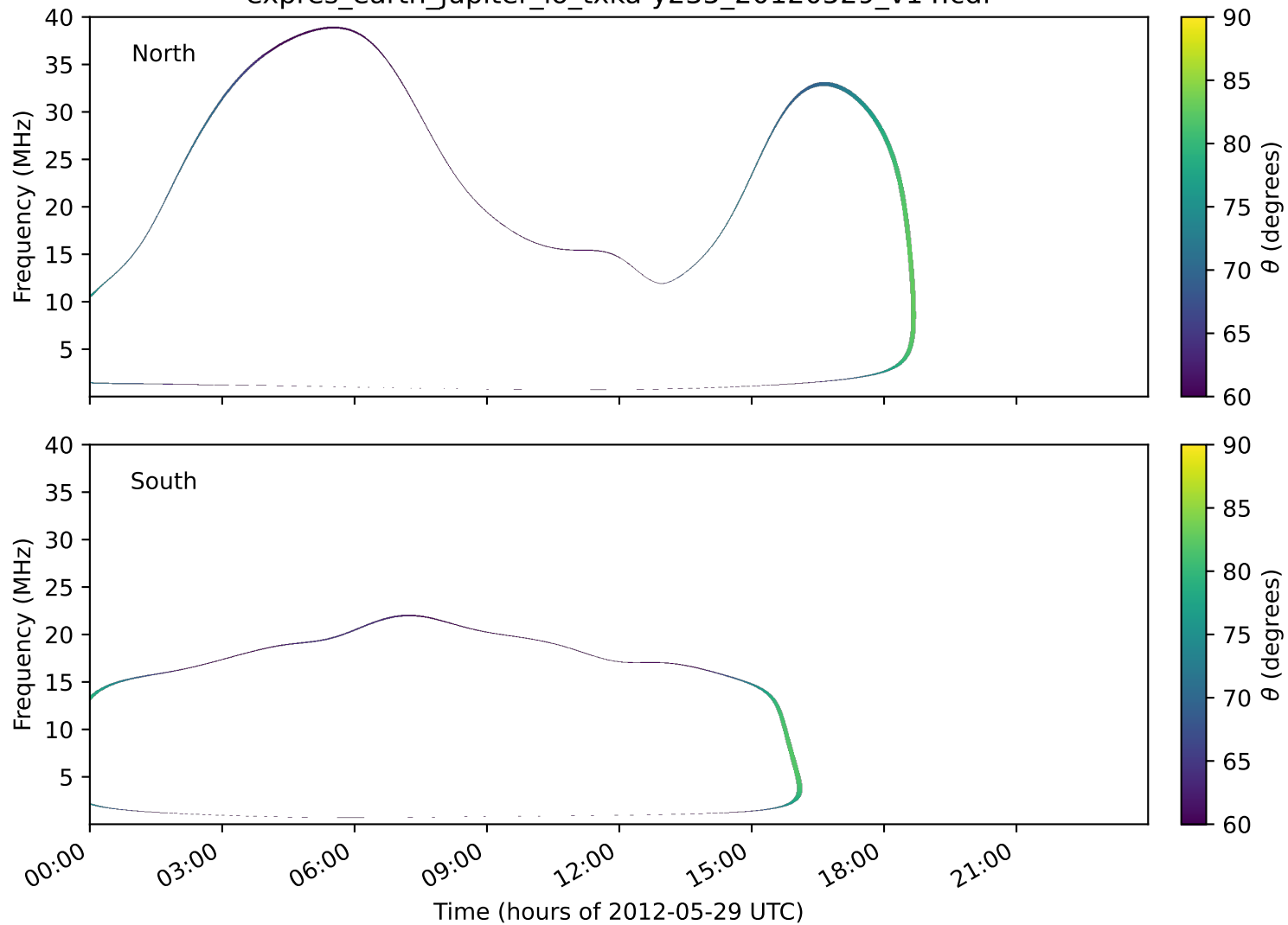
expres_earth_jupiter_io_txka-y235_20120529_v14.cdf
