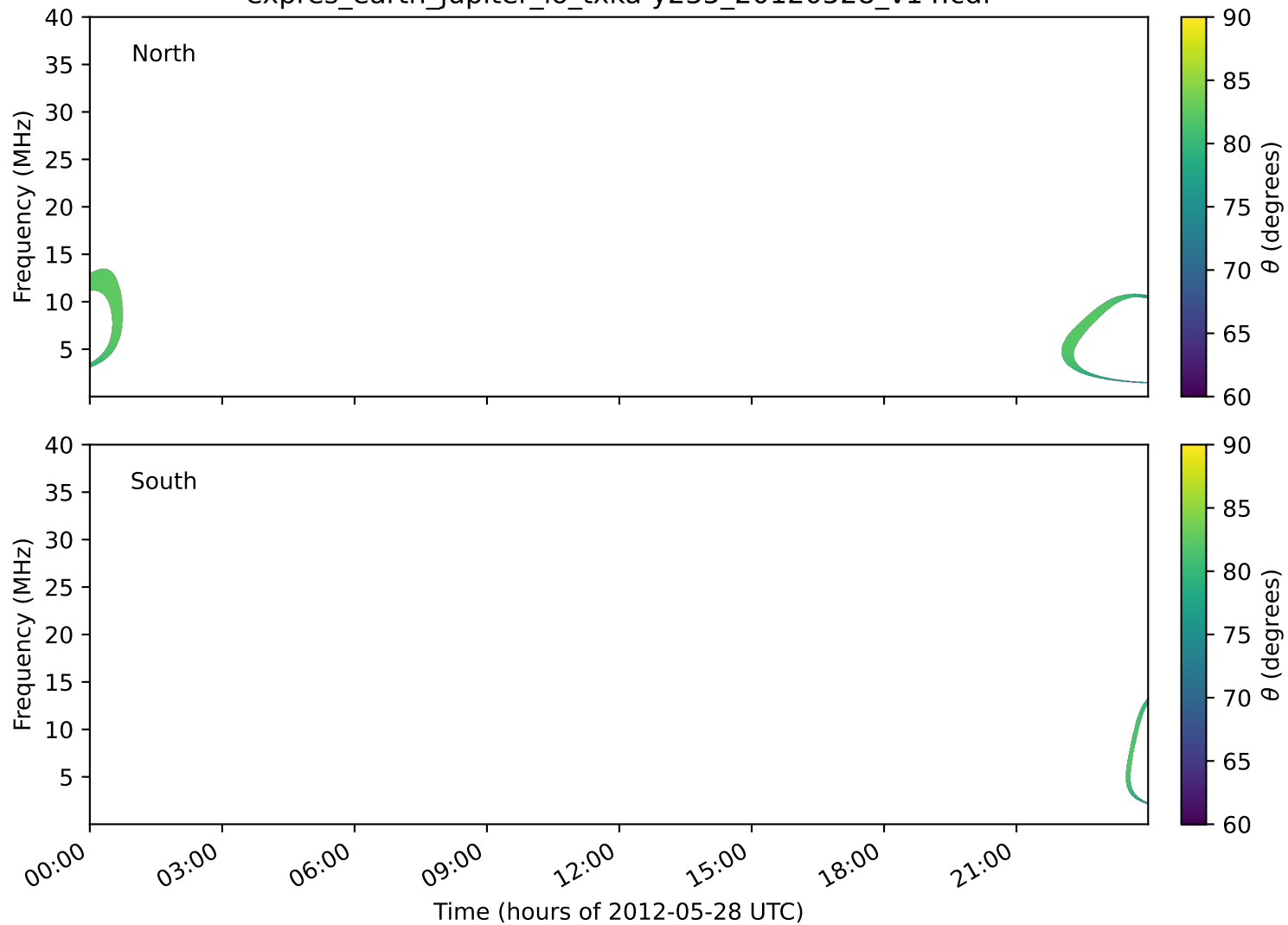
expres_earth_jupiter_io_txka-y235_20120528_v14.cdf
