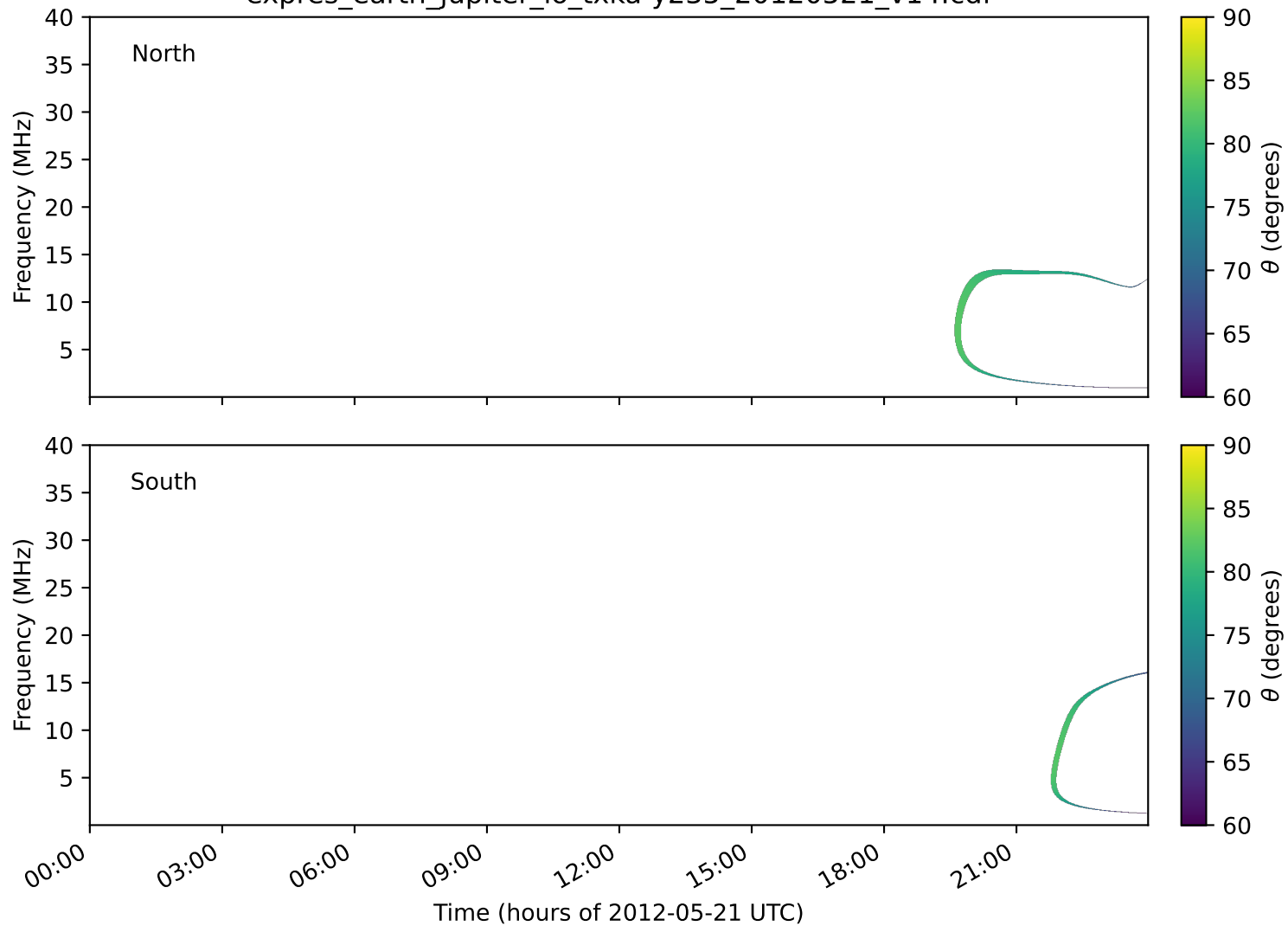
expres_earth_jupiter_io_txka-y235_20120521_v14.cdf
