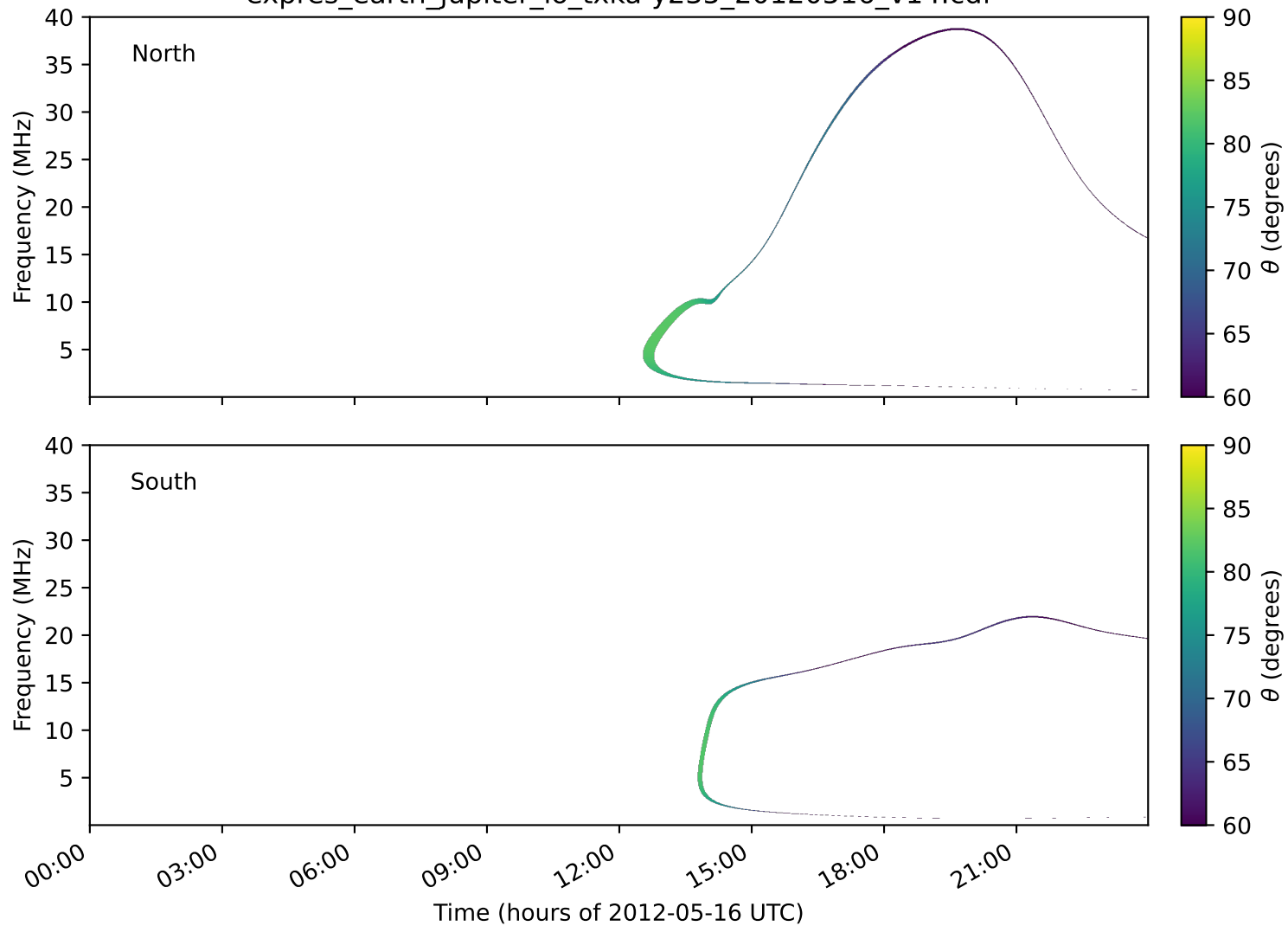
expres_earth_jupiter_io_txka-y235_20120516_v14.cdf
