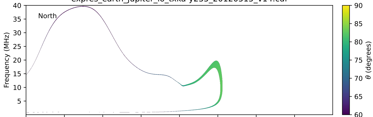
expres_earth_jupiter_io_txka-y235_20120515_v14.cdf
