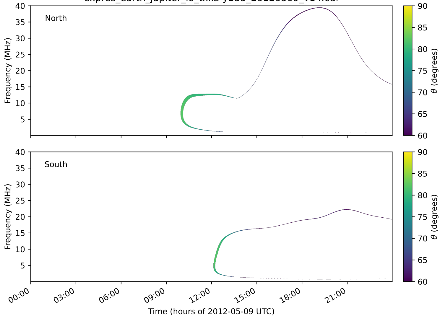
expres_earth_jupiter_io_txka-y235_20120509_v14.cdf
