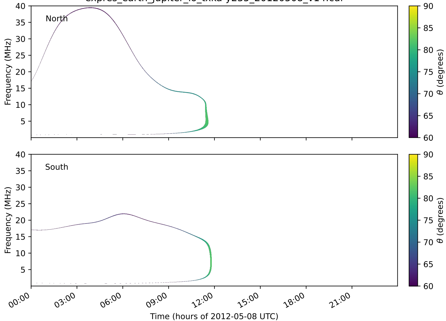
expres_earth_jupiter_io_txka-y235_20120508_v14.cdf
