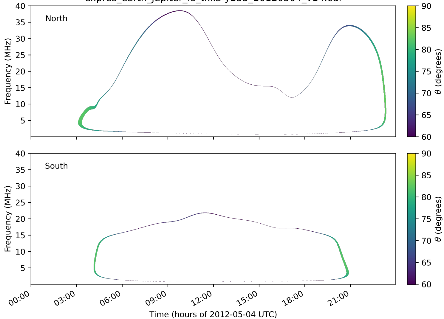
expres_earth_jupiter_io_txka-y235_20120504_v14.cdf
