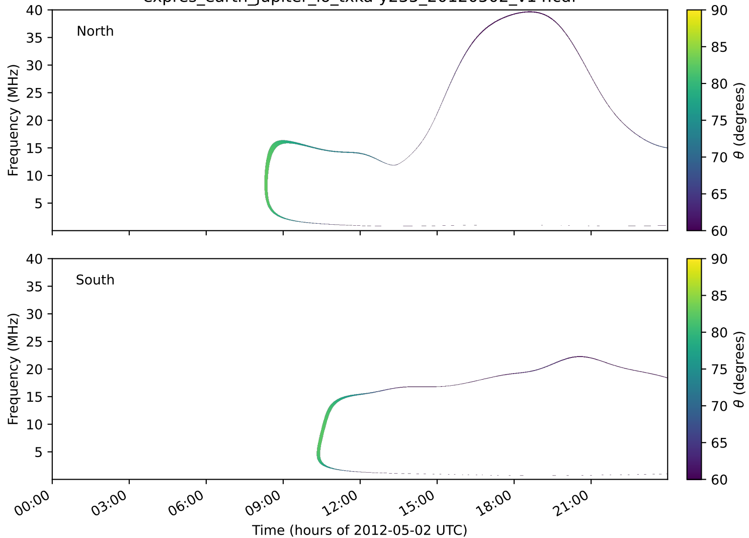
expres_earth_jupiter_io_txka-y235_20120502_v14.cdf
