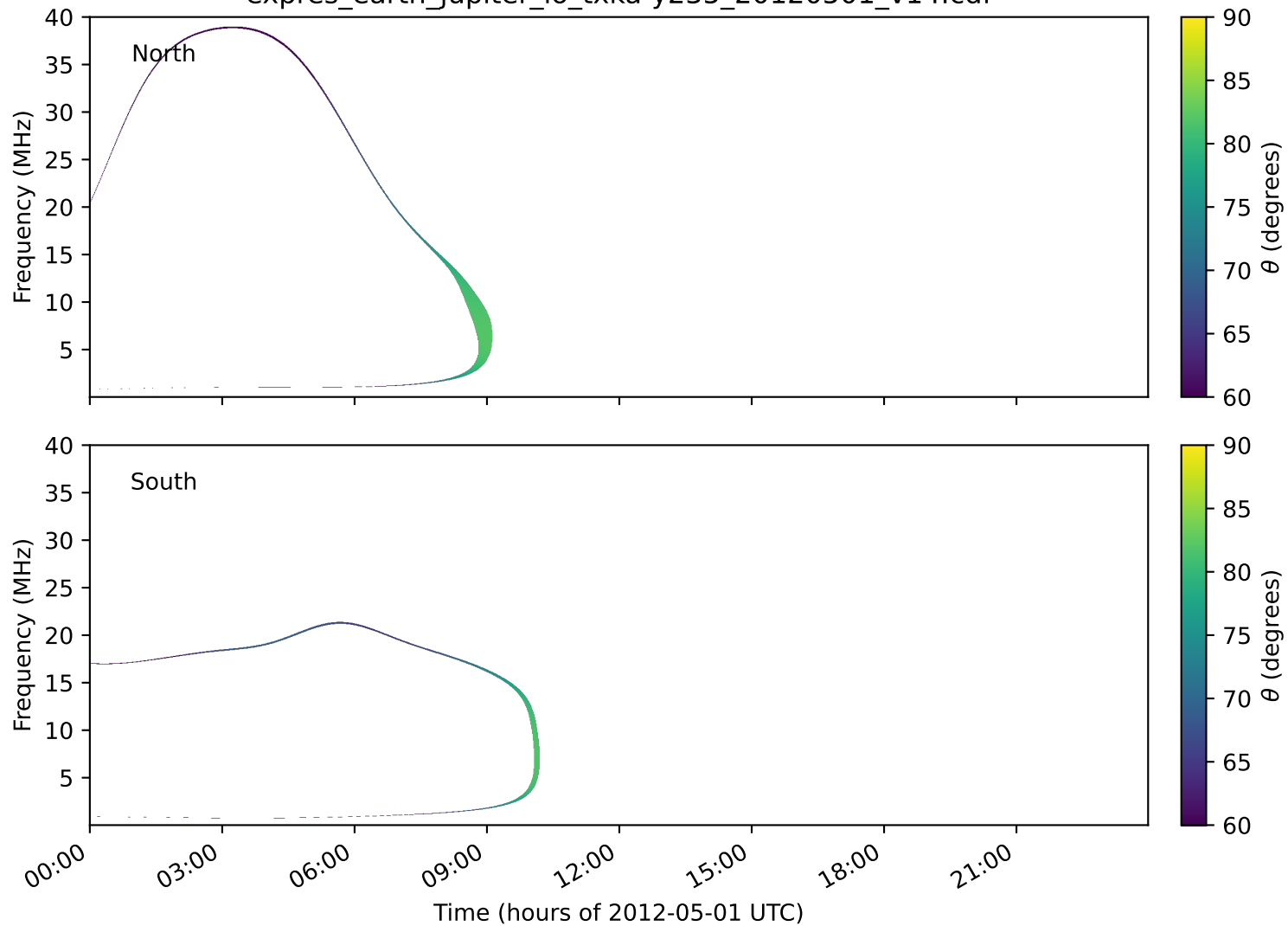
expres_earth_jupiter_io_txka-y235_20120501_v14.cdf
