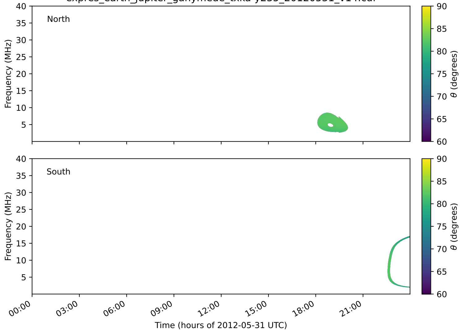
expres_earth_jupiter_ganymede_txka-y235_20120531_v14.cdf
