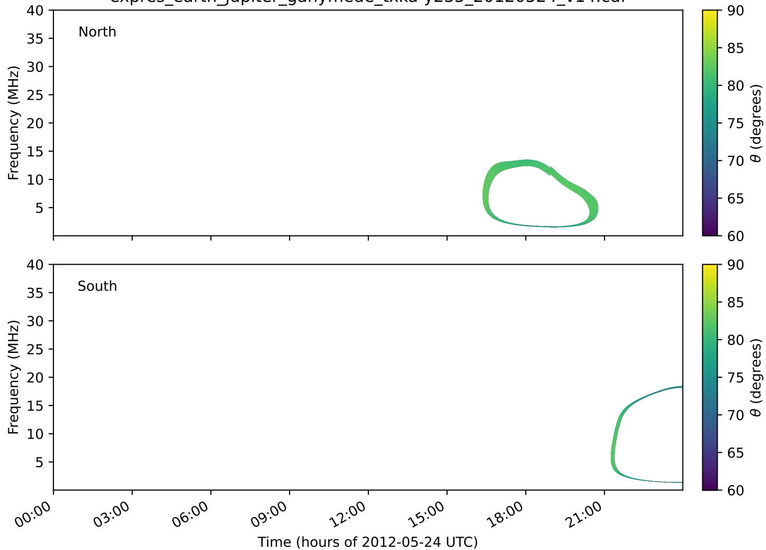
expres_earth_jupiter_ganymede_txka-y235_20120524_v14.cdf
