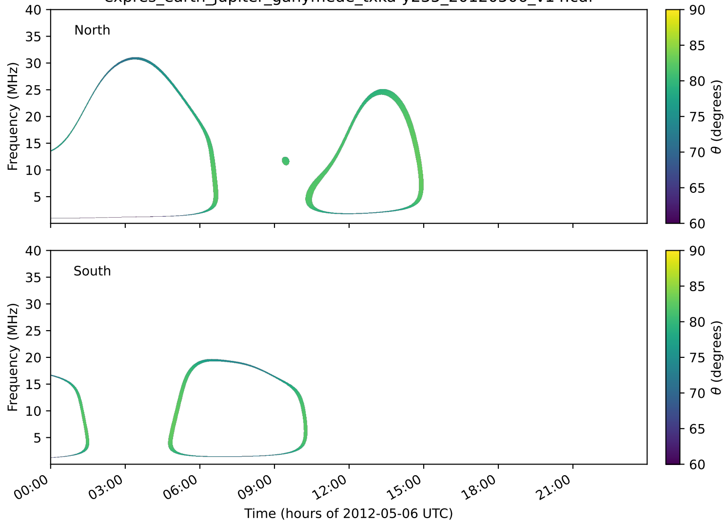
expres_earth_jupiter_ganymede_txka-y235_20120506_v14.cdf
