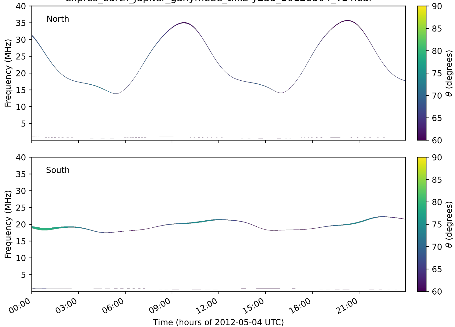
expres_earth_jupiter_ganymede_txka-y235_20120504_v14.cdf
