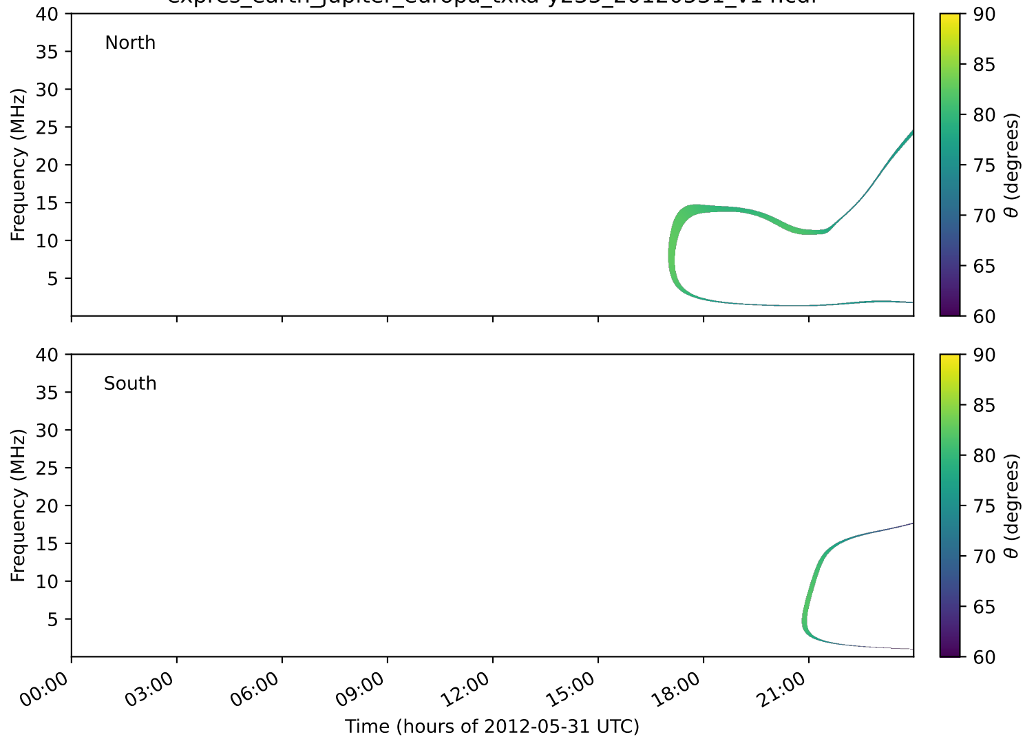
expres_earth_jupiter_europa_txka-y235_20120531_v14.cdf
