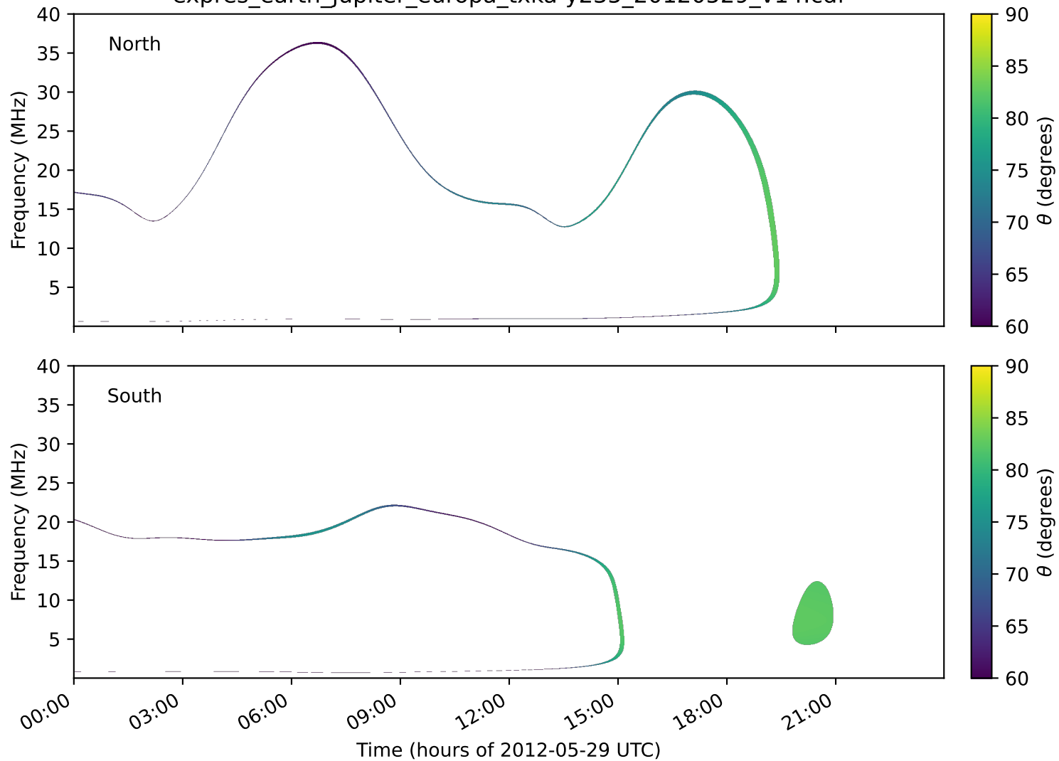
expres_earth_jupiter_europa_txka-y235_20120529_v14.cdf
