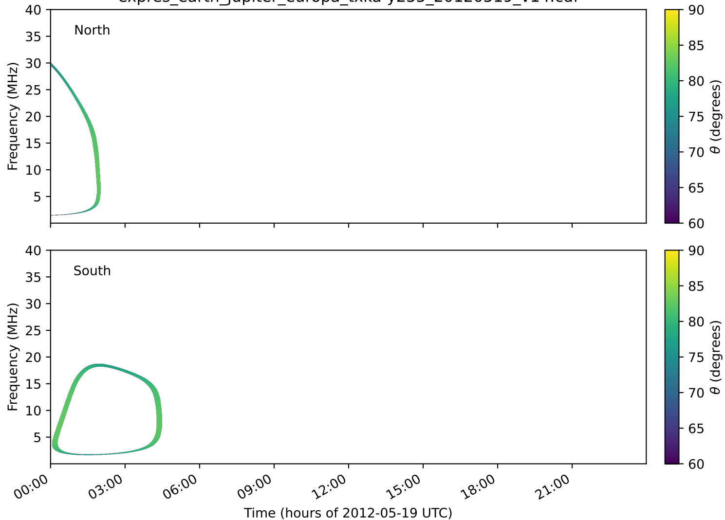
expres_earth_jupiter_europa_txka-y235_20120519_v14.cdf
