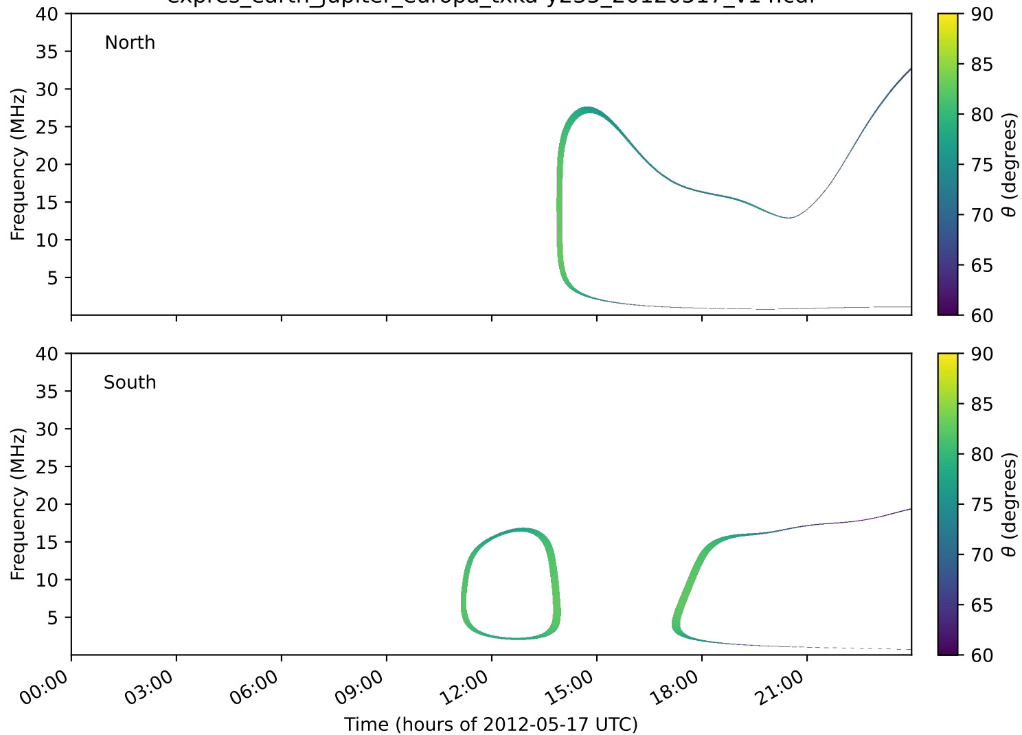
expres_earth_jupiter_europa_txka-y235_20120517_v14.cdf
