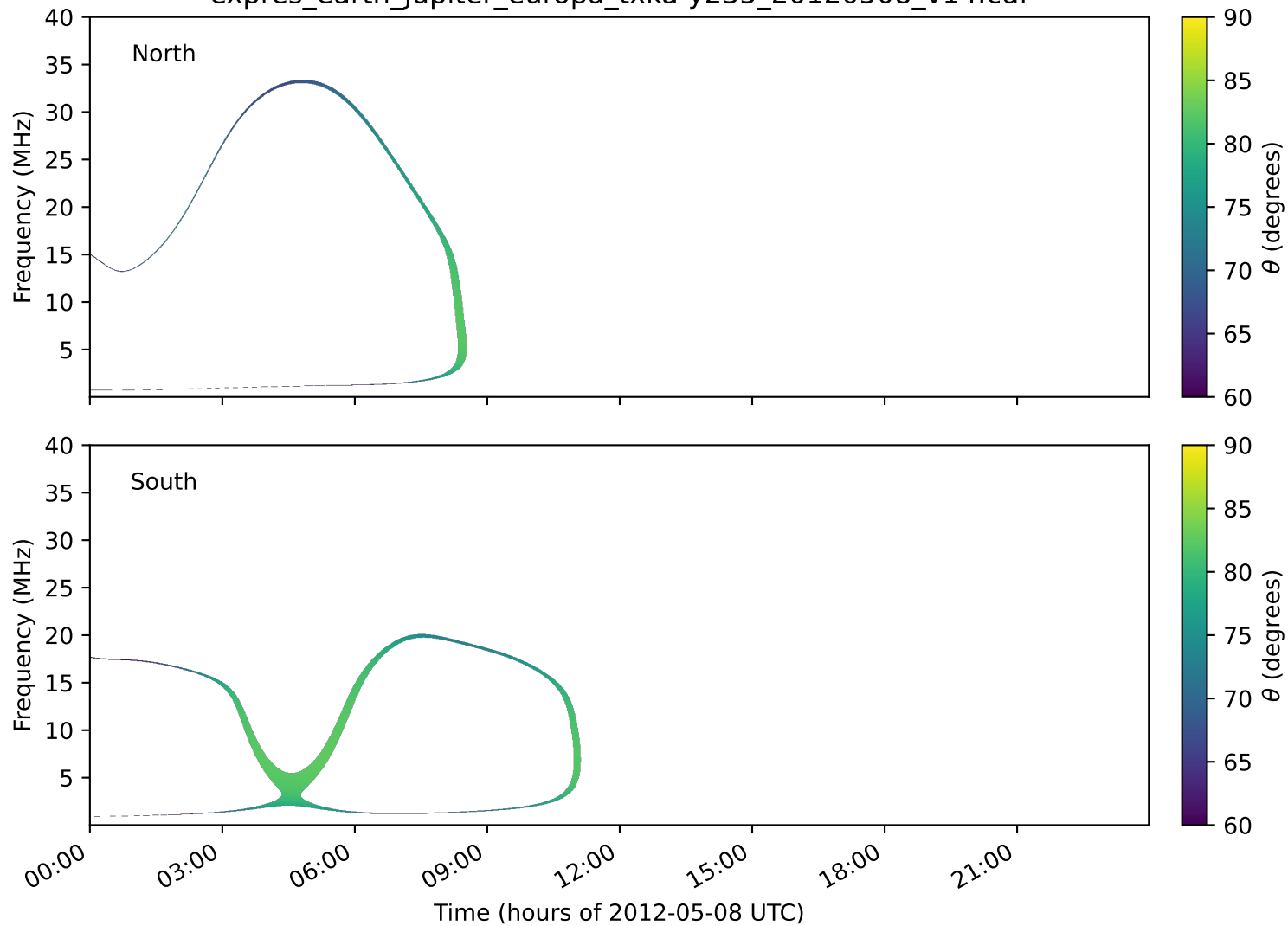
expres_earth_jupiter_europa_txka-y235_20120508_v14.cdf
