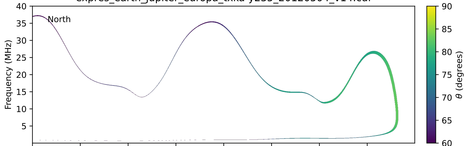
expres_earth_jupiter_europa_txka-y235_20120504_v14.cdf
