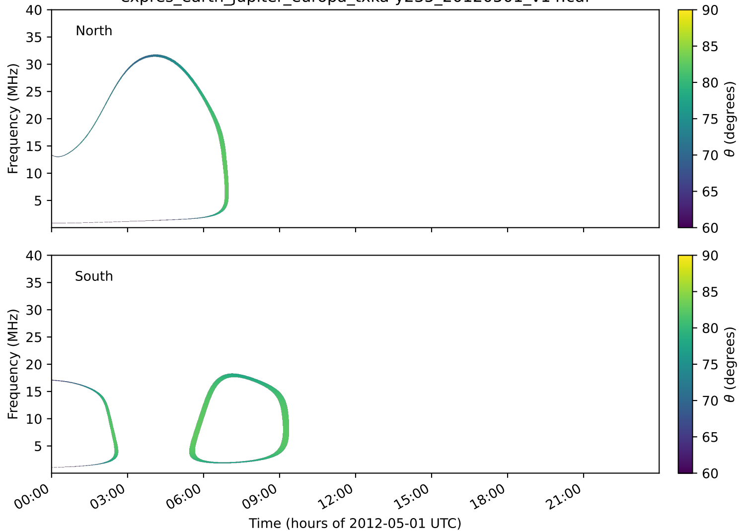
expres_earth_jupiter_europa_txka-y235_20120501_v14.cdf
