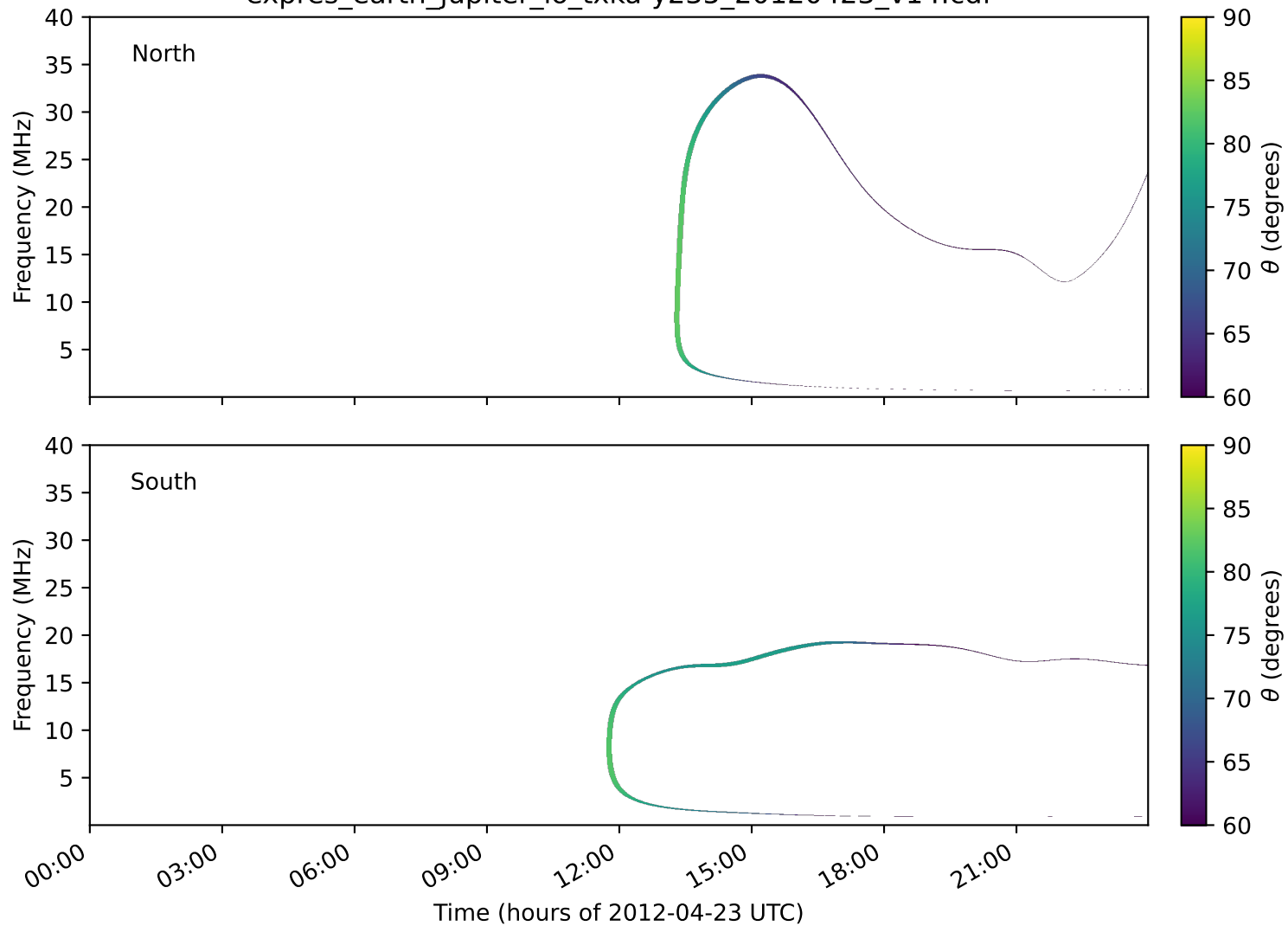
expres_earth_jupiter_io_txka-y235_20120423_v14.cdf
