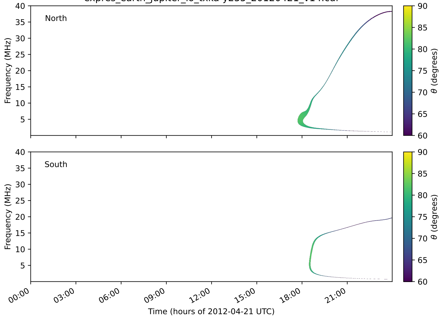
expres_earth_jupiter_io_txka-y235_20120421_v14.cdf
