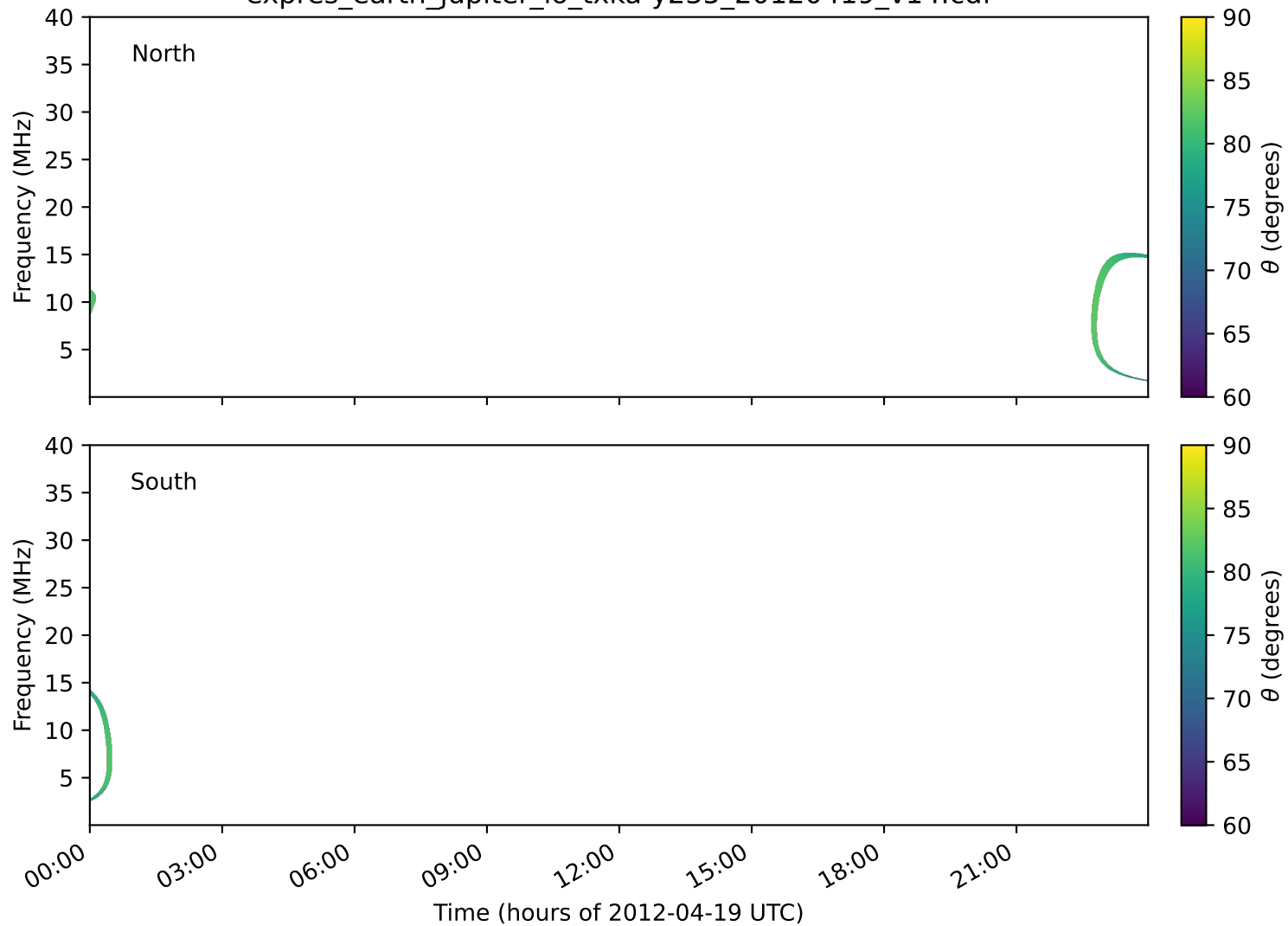
expres_earth_jupiter_io_txka-y235_20120419_v14.cdf
