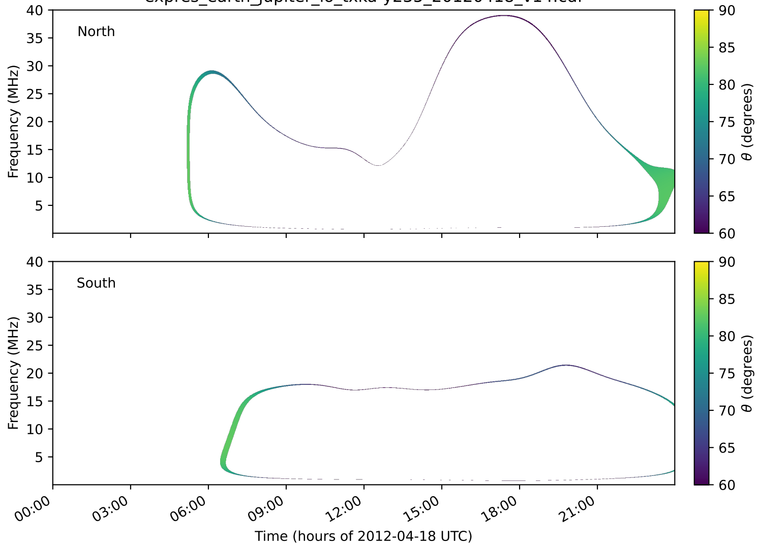
expres_earth_jupiter_io_txka-y235_20120418_v14.cdf
