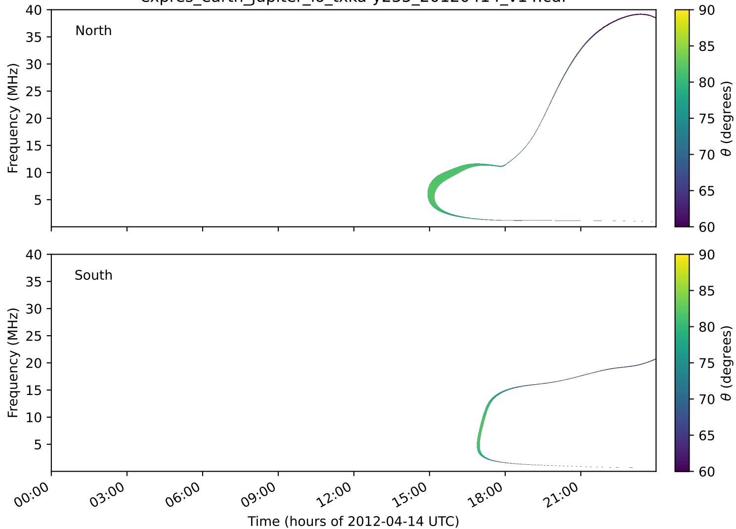
expres_earth_jupiter_io_txka-y235_20120414_v14.cdf
