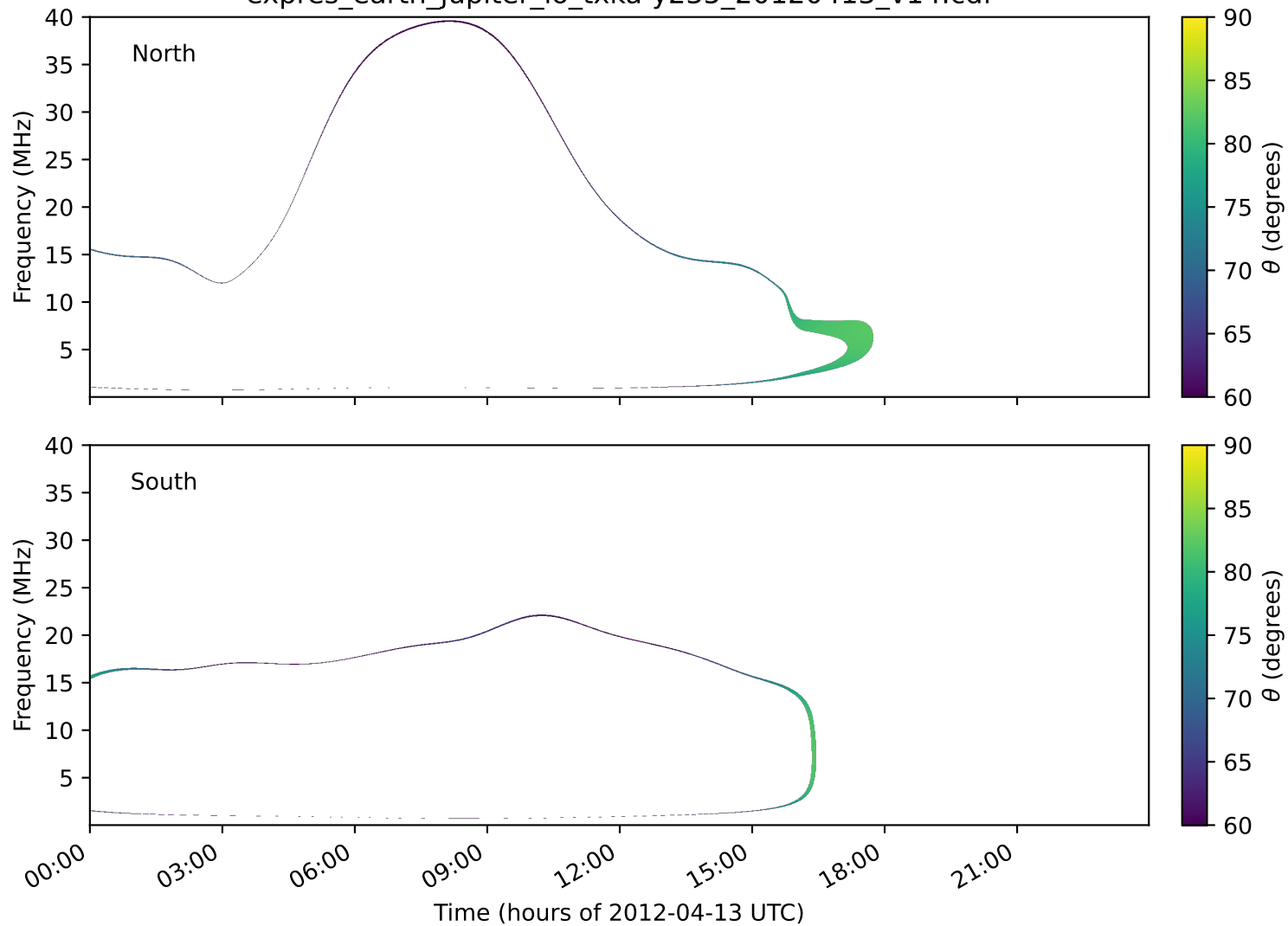
expres_earth_jupiter_io_txka-y235_20120413_v14.cdf
