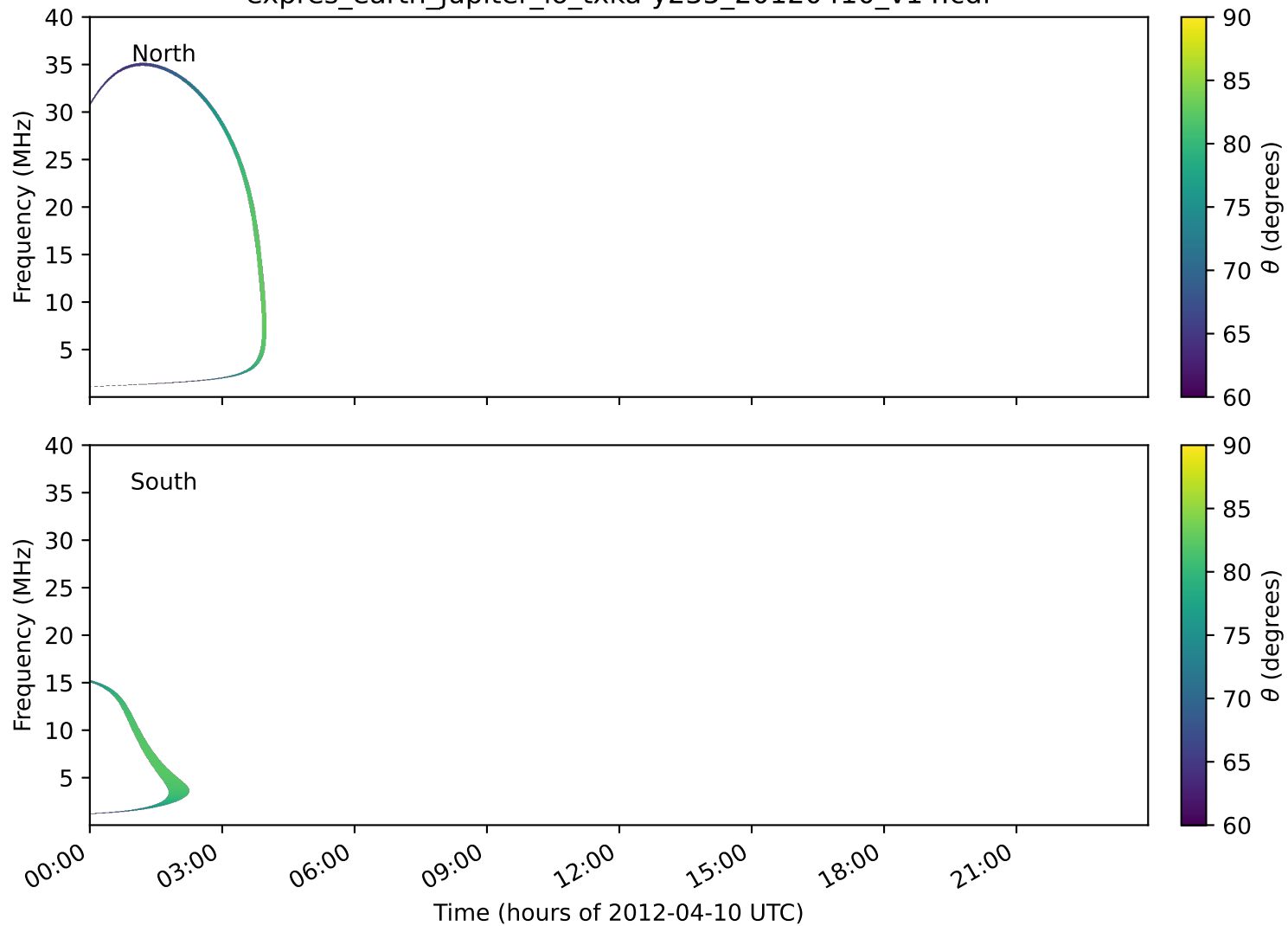
expres_earth_jupiter_io_txka-y235_20120410_v14.cdf
