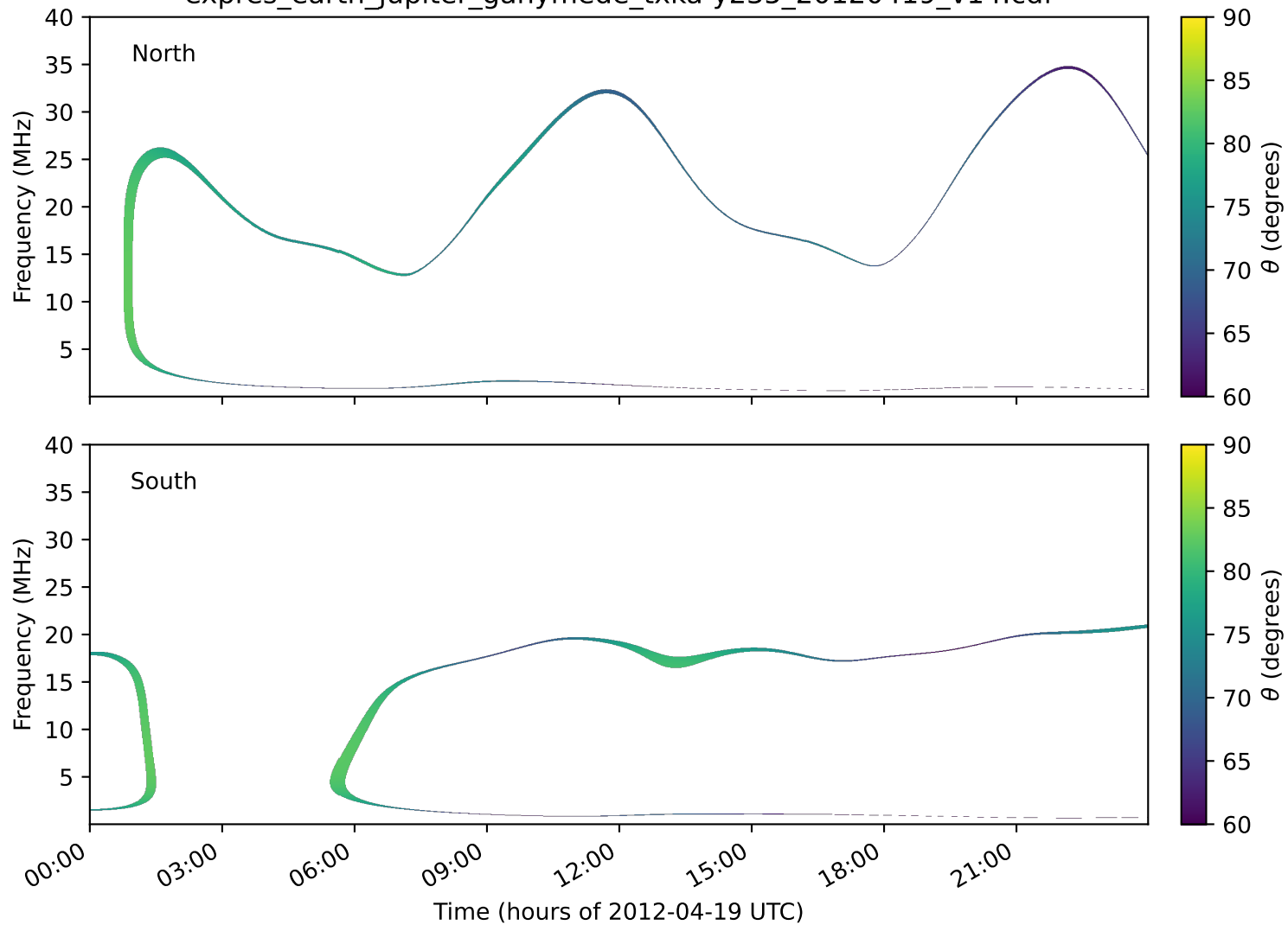
expres_earth_jupiter_ganymede_txka-y235_20120419_v14.cdf
