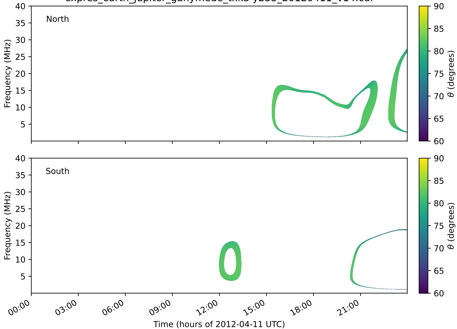
expres_earth_jupiter_ganymede_txka-y235_20120411_v14.cdf
