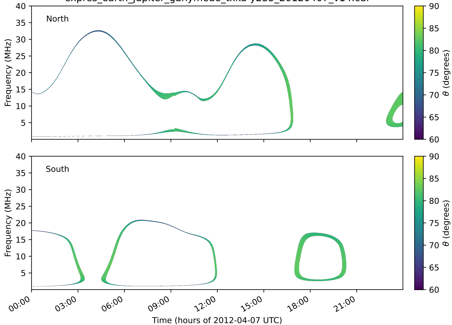
expres_earth_jupiter_ganymede_txka-y235_20120407_v14.cdf
